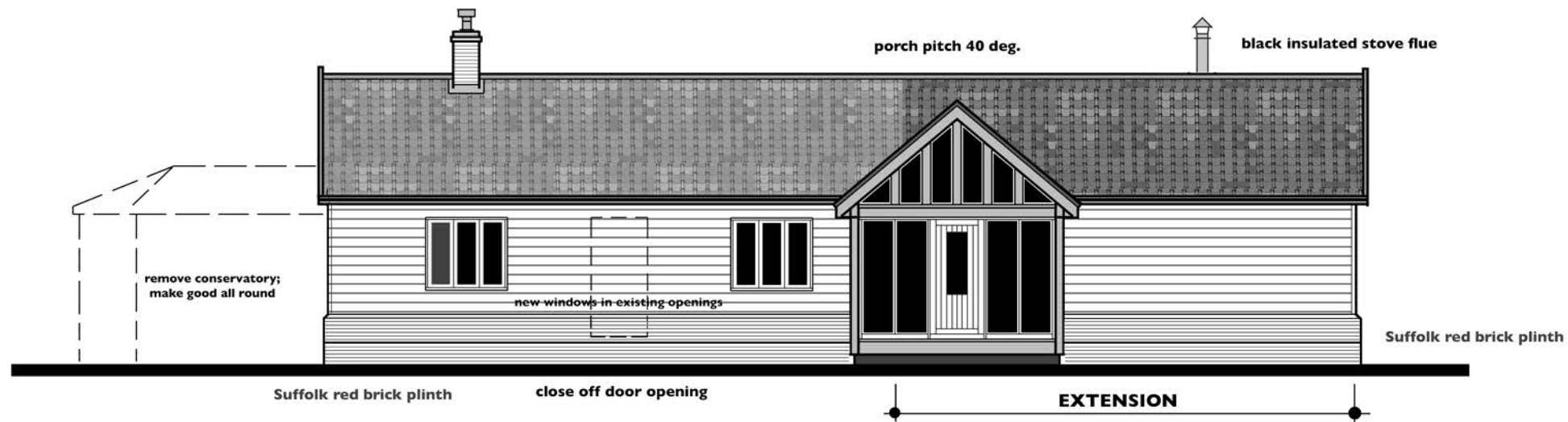
:: Front (East) :: Proposed :: 1:100 ::
