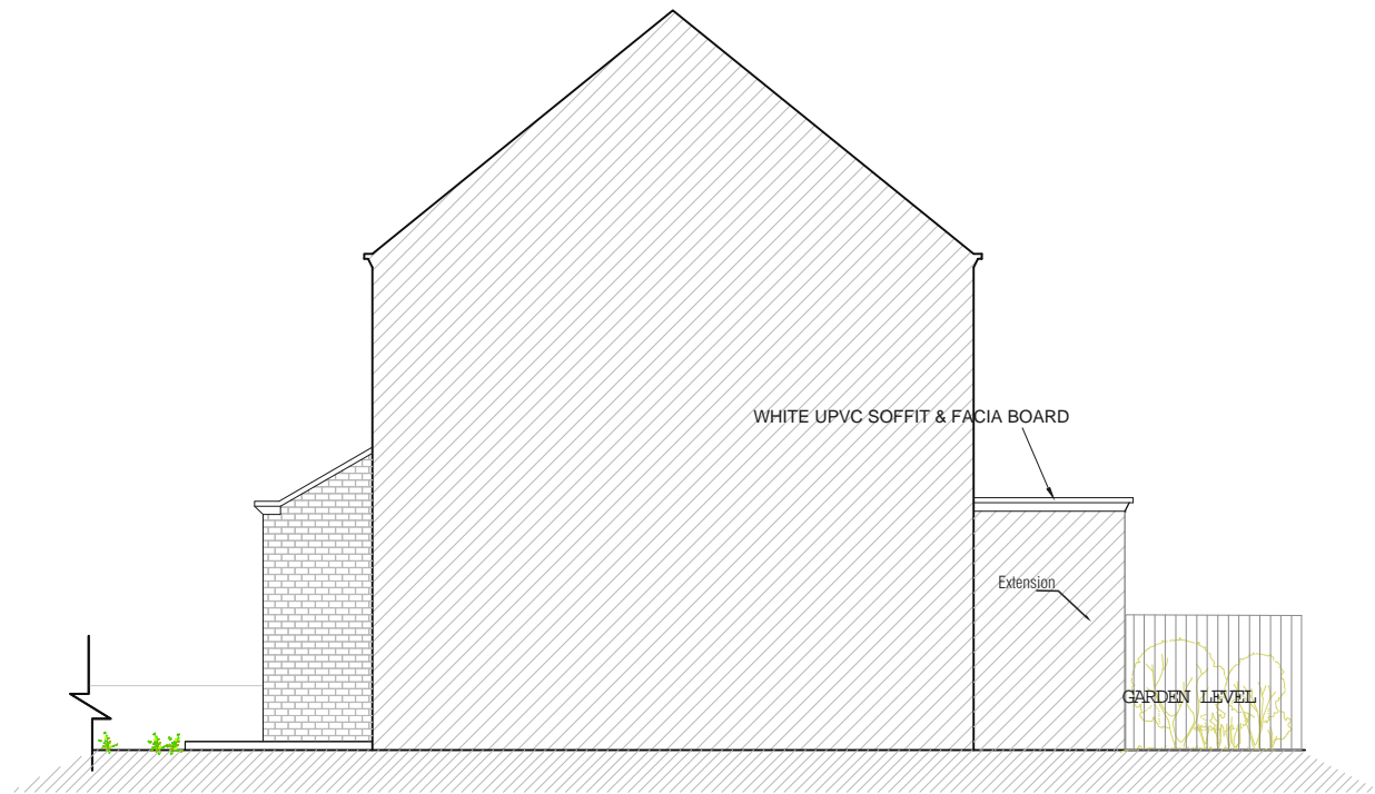
PROPOSED SIDE ELEVATION VIEW A SCALE 1:100
