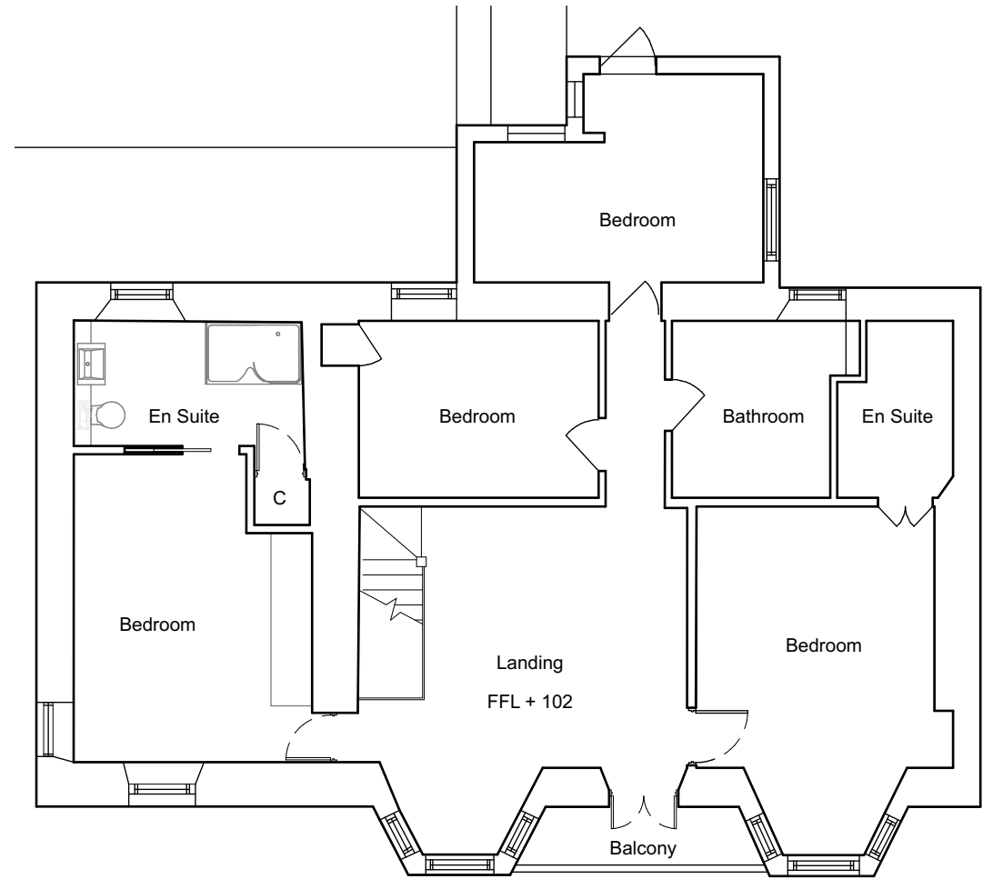
EXISTING FRIST FLOOR PLAN 1:100
