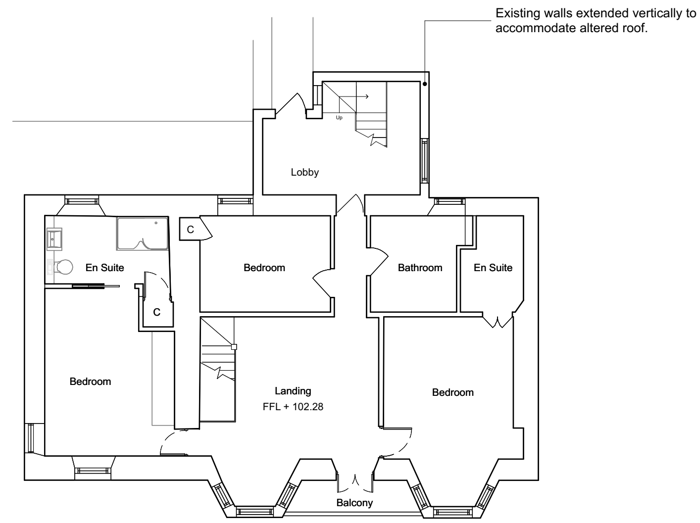
PROPOSED FRIST FLOOR PLAN 1:100
