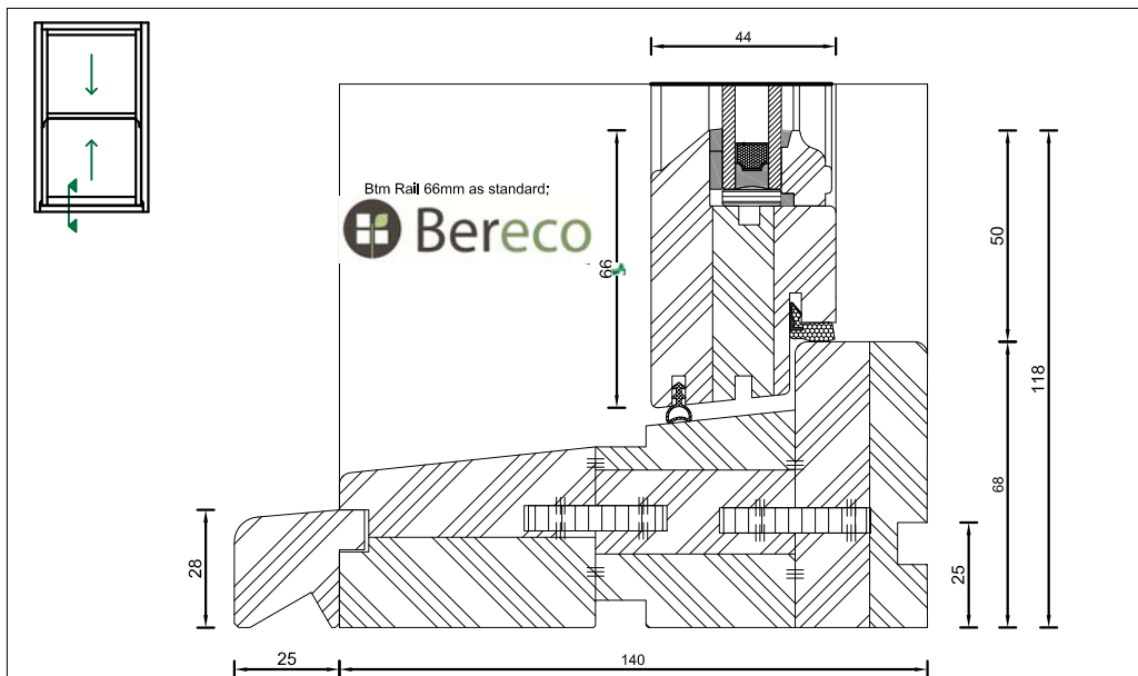
Heritage Slim-Line Sliding Sash Spiral Balance Frame & Sash Cill
