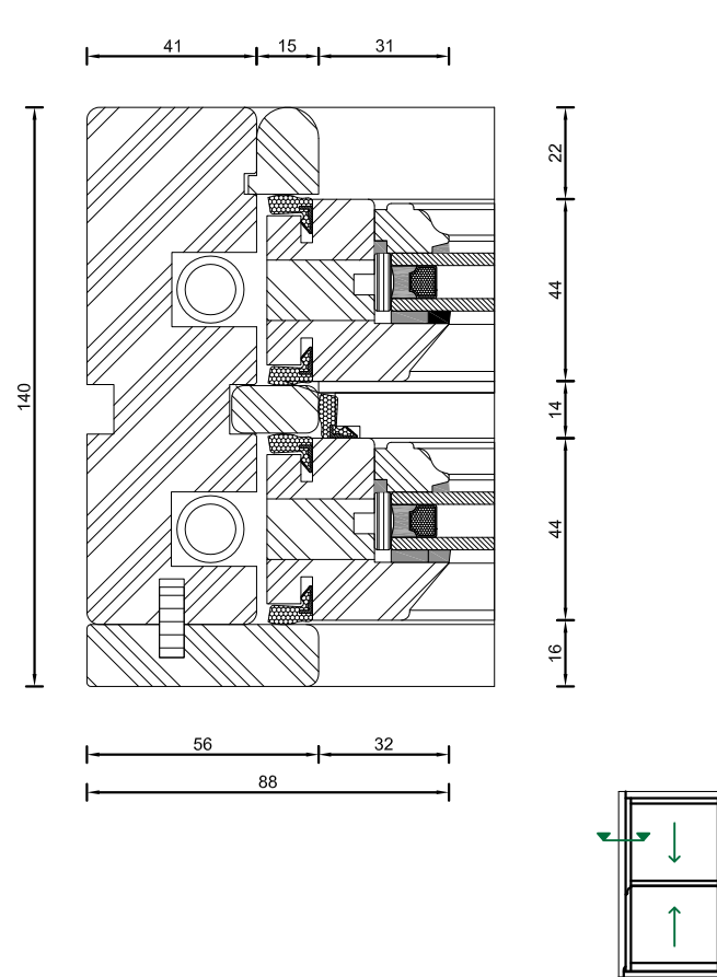
Heritage Slim-Line Sliding Sash Spiral Balance Frame & Sash Jamb
