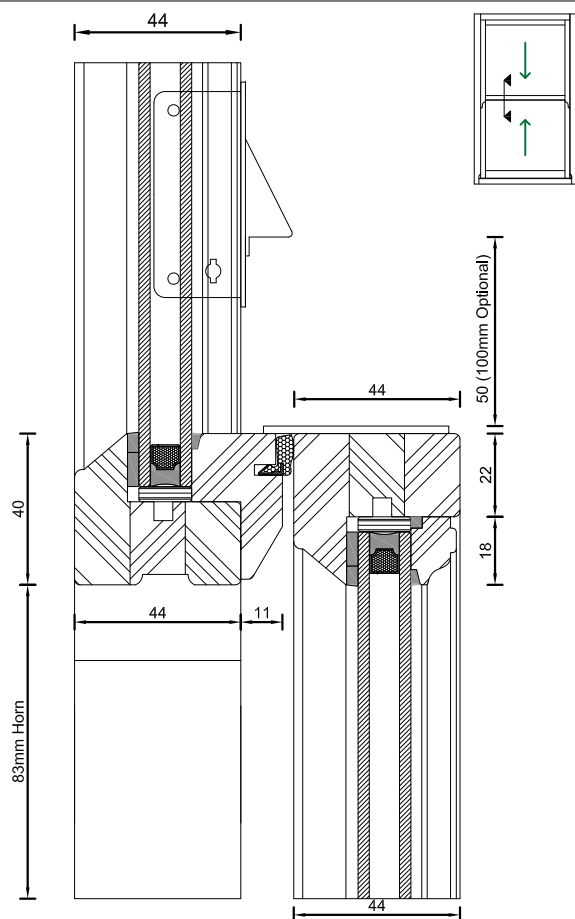
Heritage Slim-Line Sliding Sash Spiral Balance Meeting Rail
