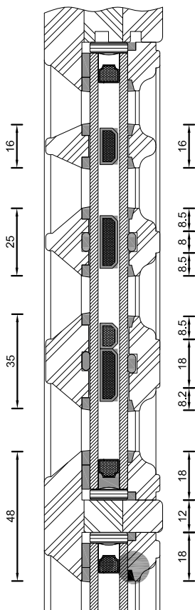
Heritage Slim-Line Sliding Sash Spiral Balance Bar Options
