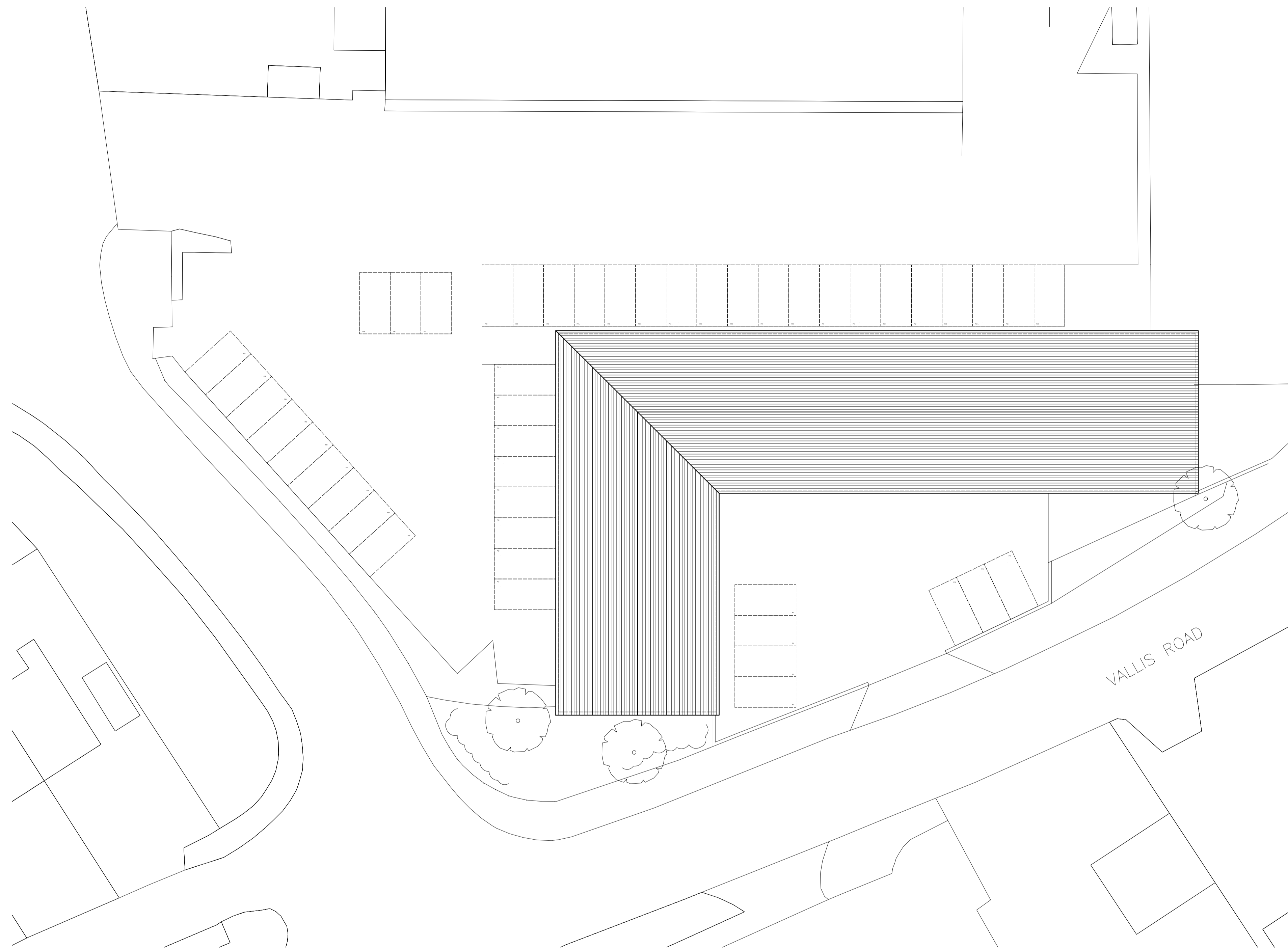
1 PROPOSED SITE PLAN SCALE - 1:200 @ A1
