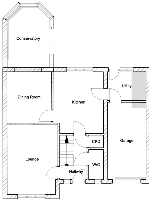
Existing Ground Floor Layout
