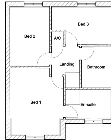
Proposed First Floor Layout
