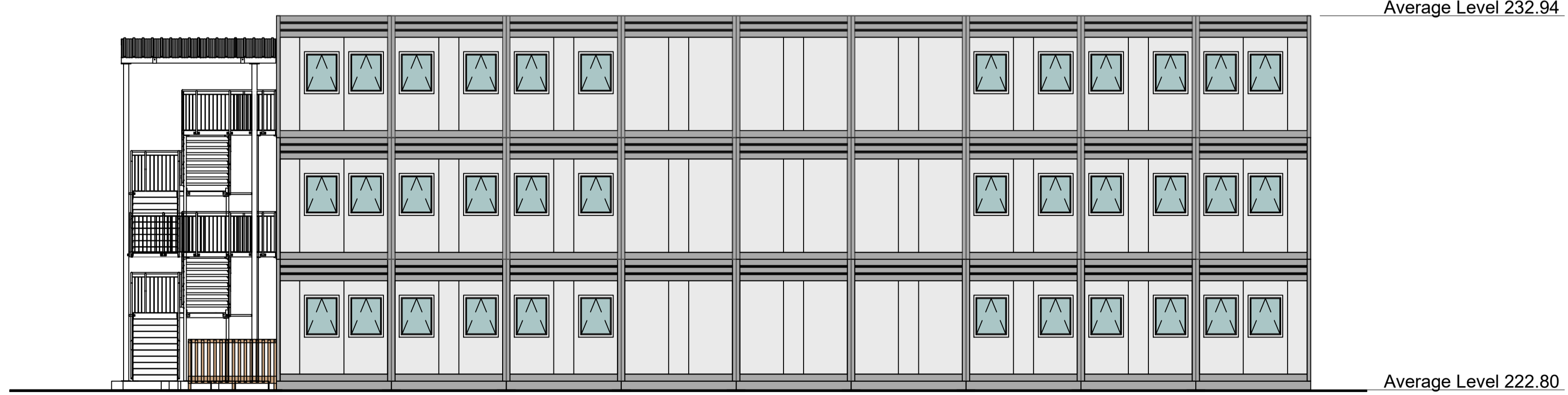
ELEVATION C - SOUTH
