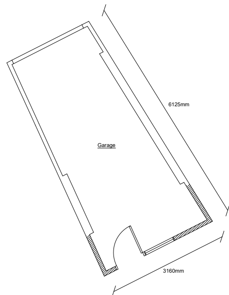
Garage Plan as Proposed 1:100
