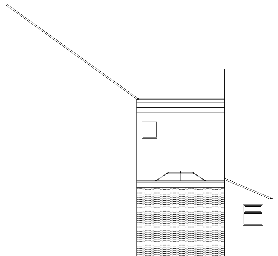
Part Side Elevation as Proposed 1:100
