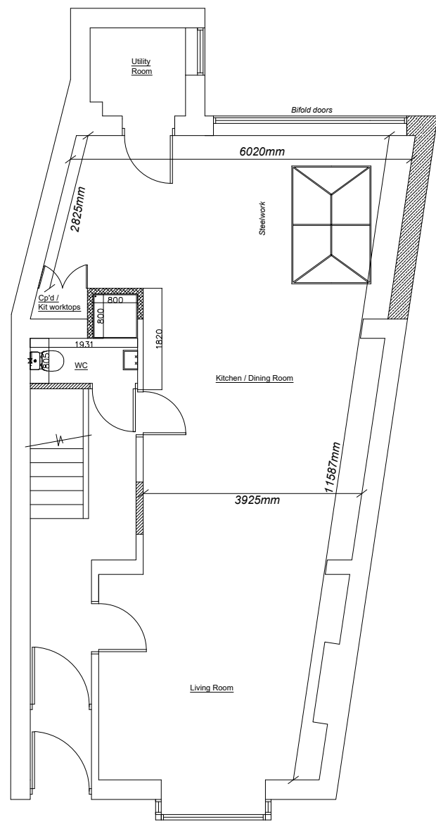
Ground Floor Plan as Proposed 1:100
