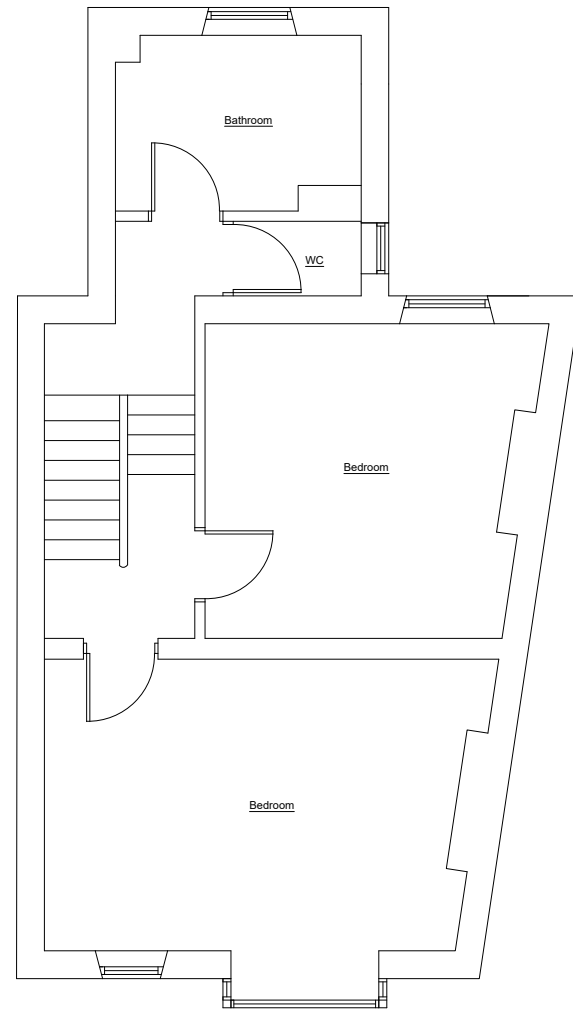
First Floor Plan as Existing 1:100
