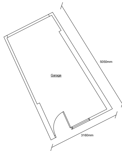
Garage Plan as Existing 1:100
