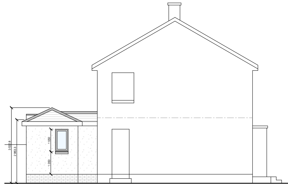
East Elevation
