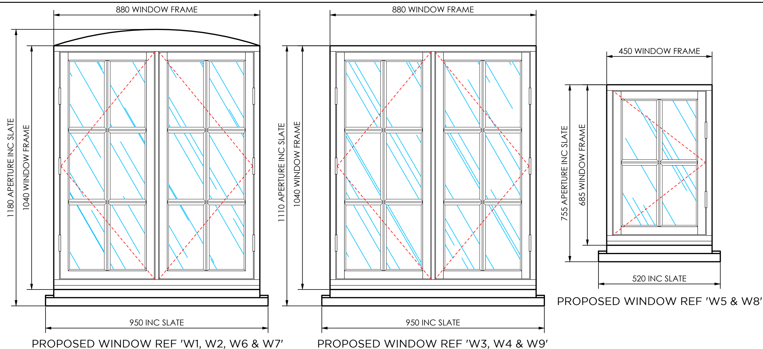
13 GENERAL WINDOW SIZES AND DESIGN STYLES AS PROPOSED (ALL REPLACEMENTS TO BE LIKE FOR LIKE) 1:10 @ A3
