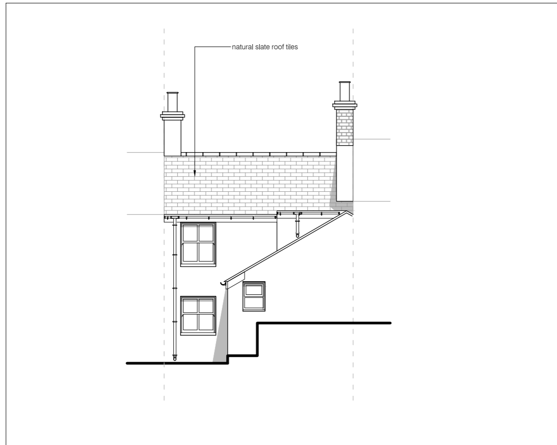
01 PROPOSED NORTH WEST ELEVATION 1:100
