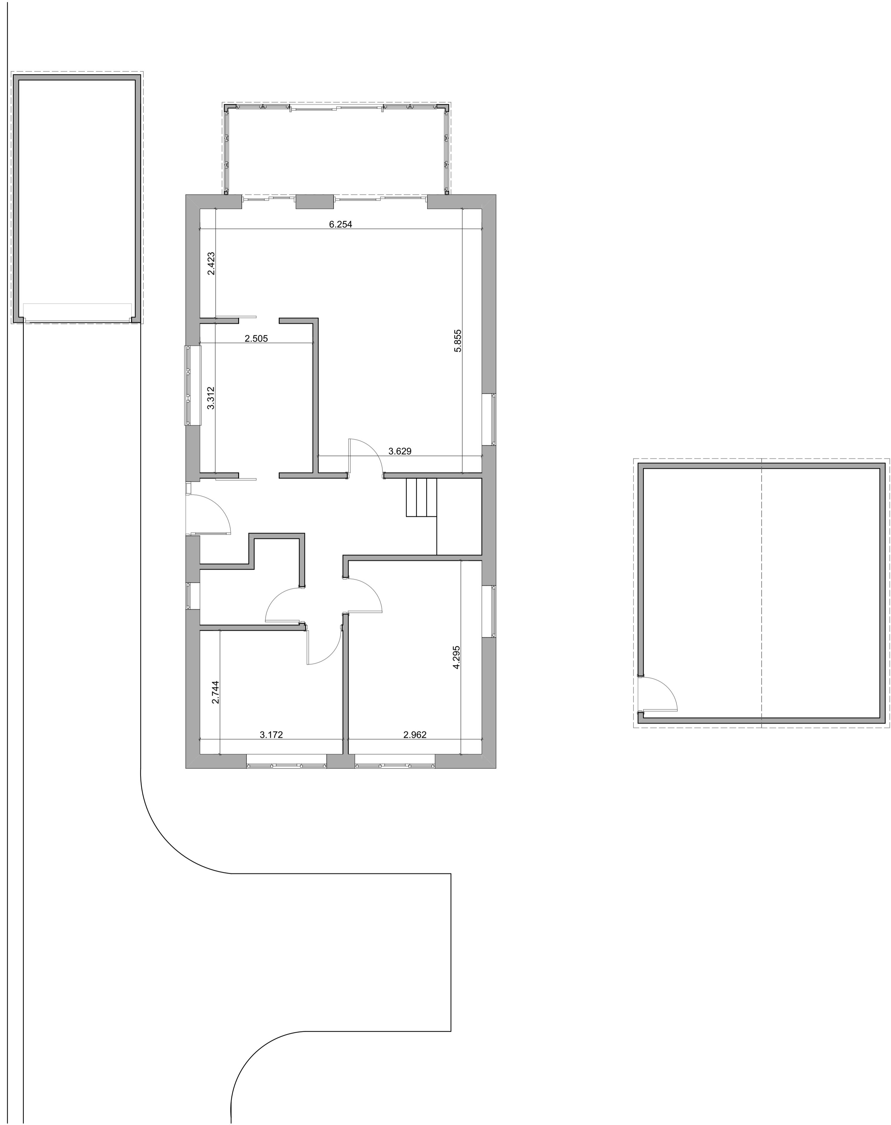
0. Ground Floor 1:50
