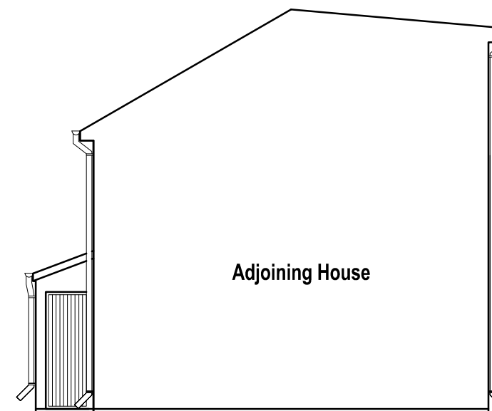
Side 2 Elevation - Proposed
