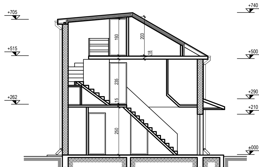
Section - Proposed
