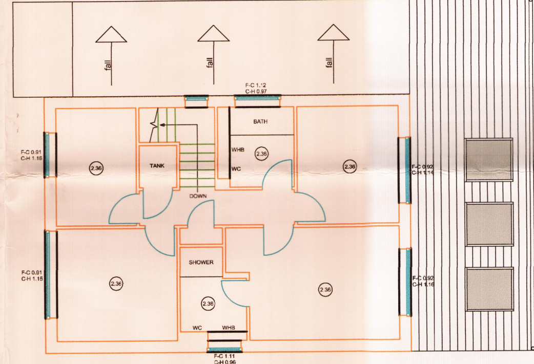
FIRST FLOOR PLAN - ROOF PLAN
