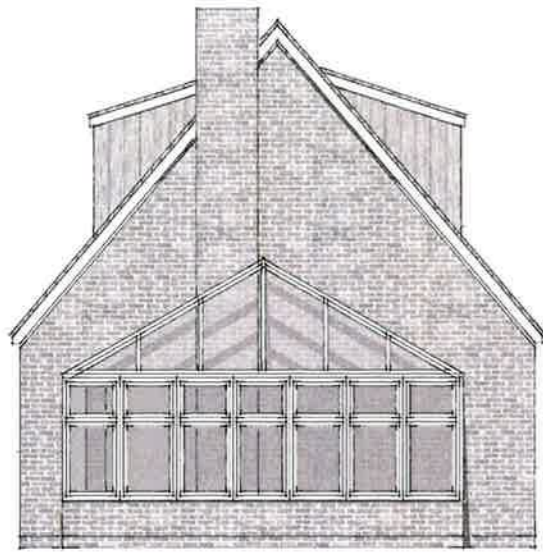
EXISTING SOUTH ELEVATION
