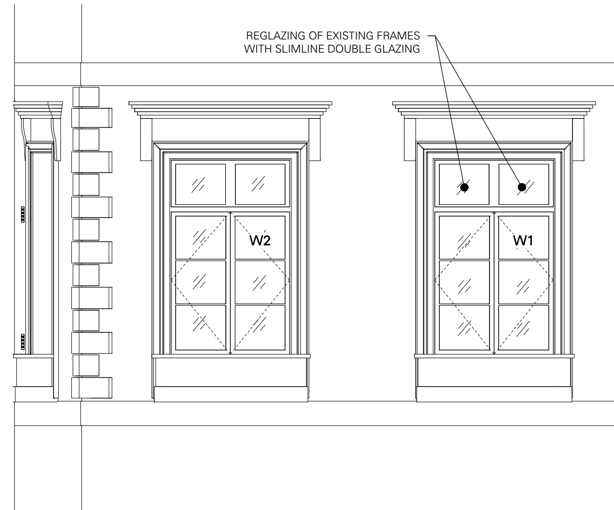
2 PROPOSED NORTH ELEVATION 1 : 50
