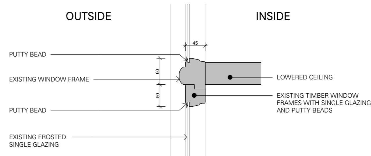
6 BATHROOM MEETING DETAIL 1 : 5
