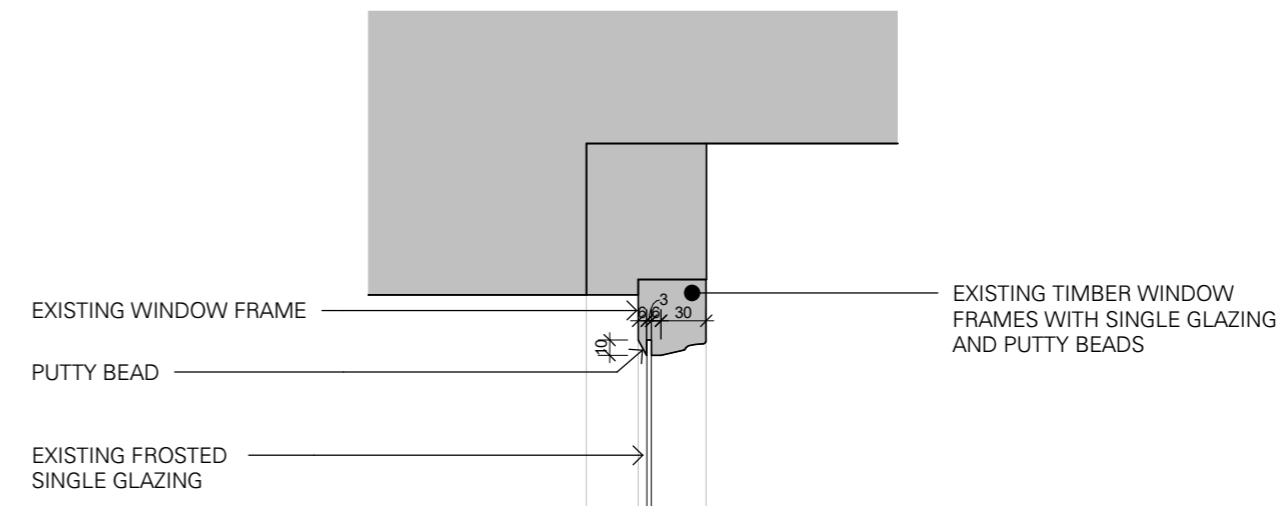
5 BATHROOM HEAD DETAIL 1 : 5
