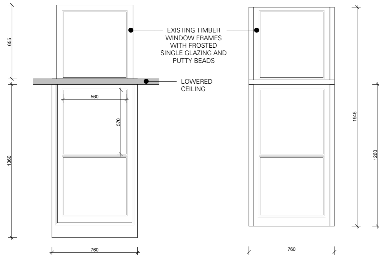
1 EXISTING INTERNAL ELEVATION 1 : 20
