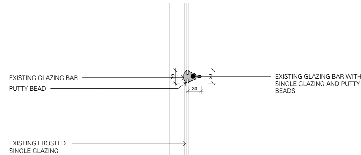
7 BATHROOM GLAZING BAR DETAIL 1 : 5
