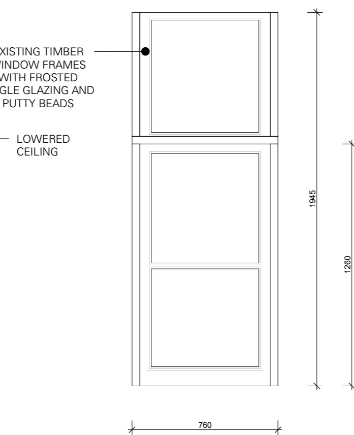
2 EXISTING EXTERNAL ELEVATION 1 : 20
