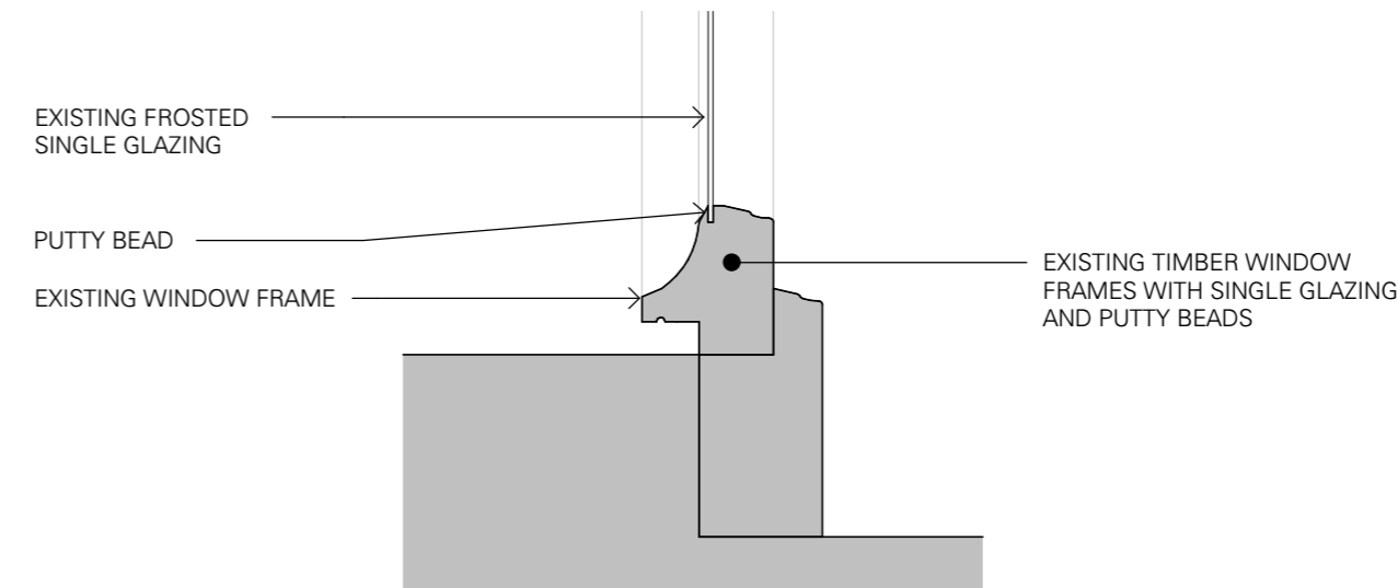
8 BATHROOM CILL DETAIL 1 : 5
