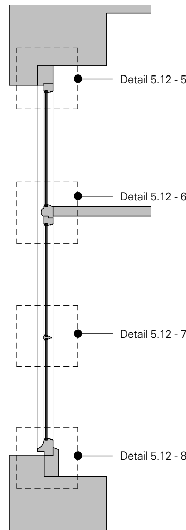
3 PROPOSED SECTION 1 : 20
