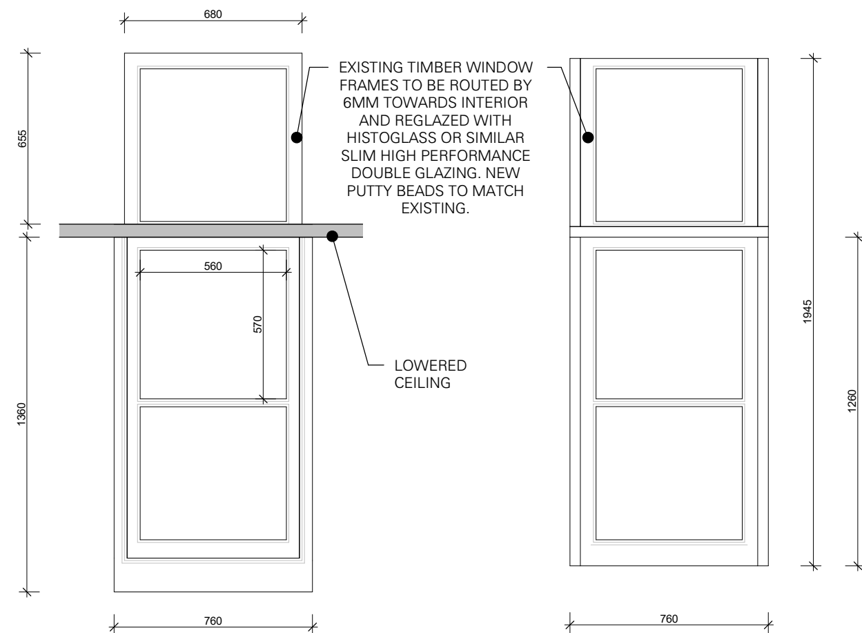
1 PROPOSED INTERNAL ELEVATION 1 : 20
