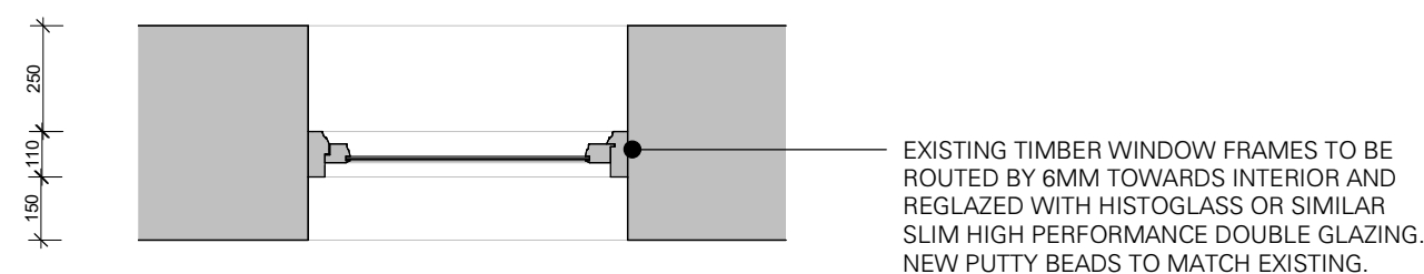
4 PROPOSED BATHROOM WINDOW PLAN 1 : 20
