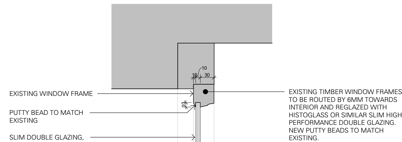
5 PROPOSED BATHROOM HEAD DETAIL 1 : 5
