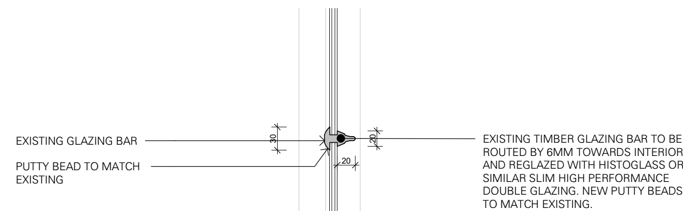
6 PROPOSED BATHROOM MEETING DETAIL 1 : 5
