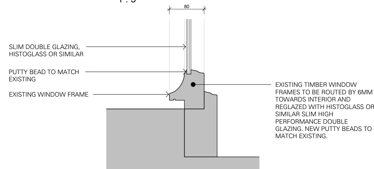
8 PROPOSED BATHROOM CILL DETAIL 1 : 5
