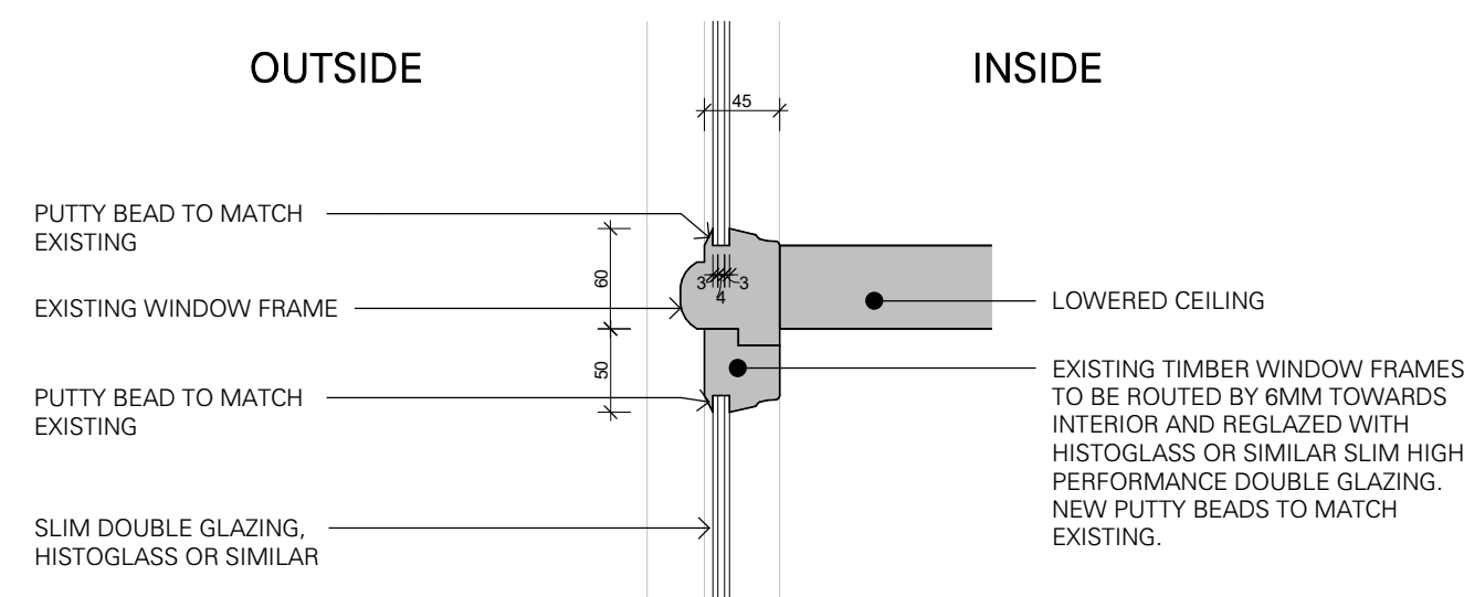
6 PROPOSED BATHROOM MEETING DETAIL 1 : 5
