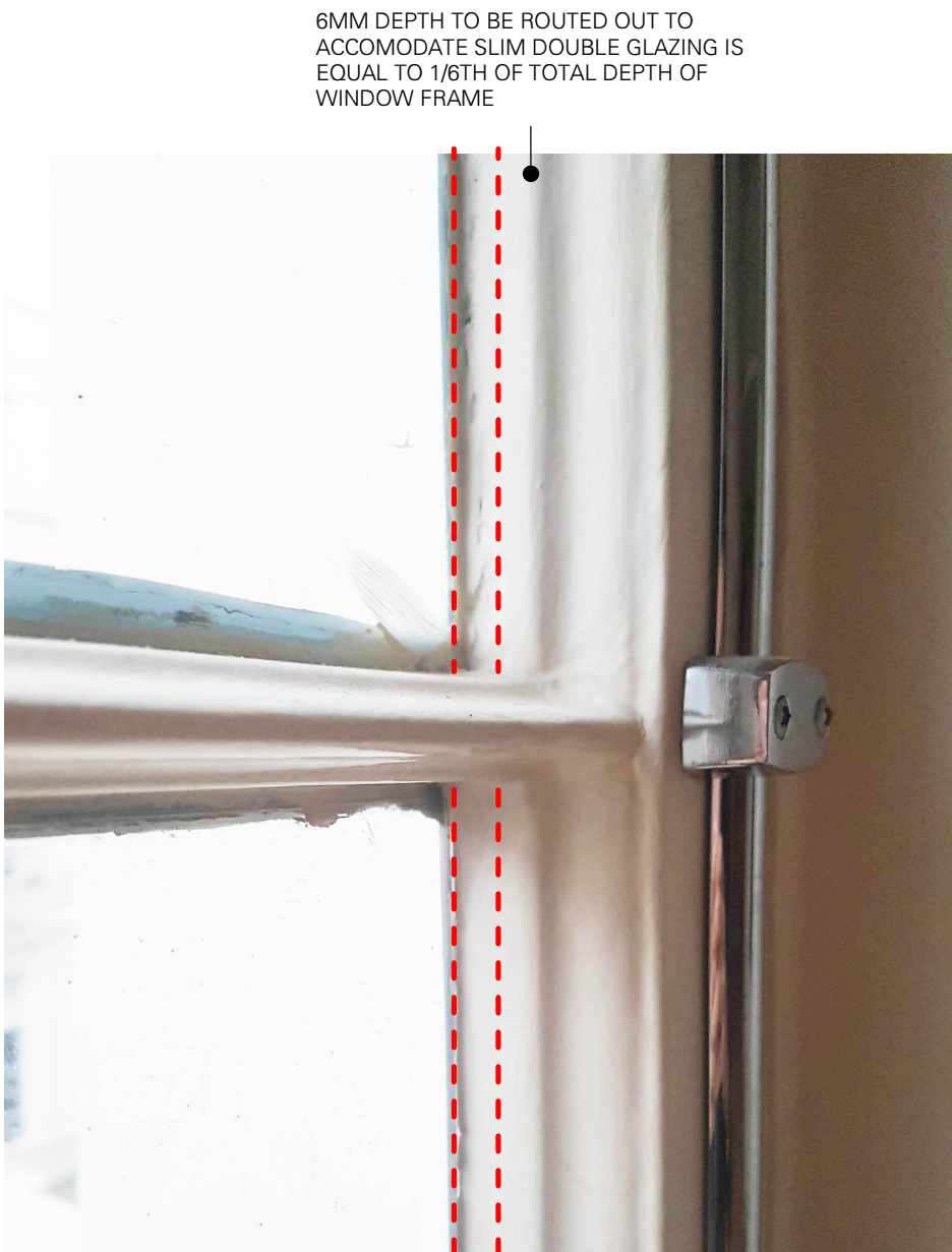
EXISTING GLAZING BAR AND WINDOW FRAME
