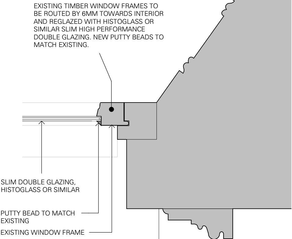
6 PROPOSED JAMB DETAIL 1 : 5
