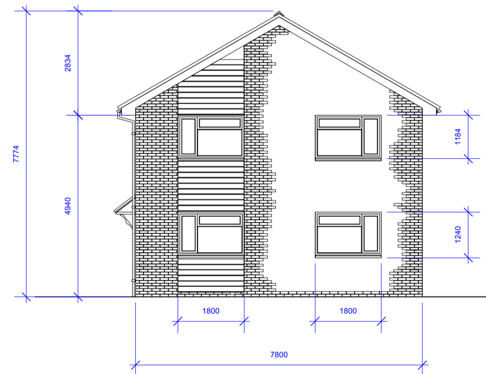
Existing right hand side elevation Scale 1:100
