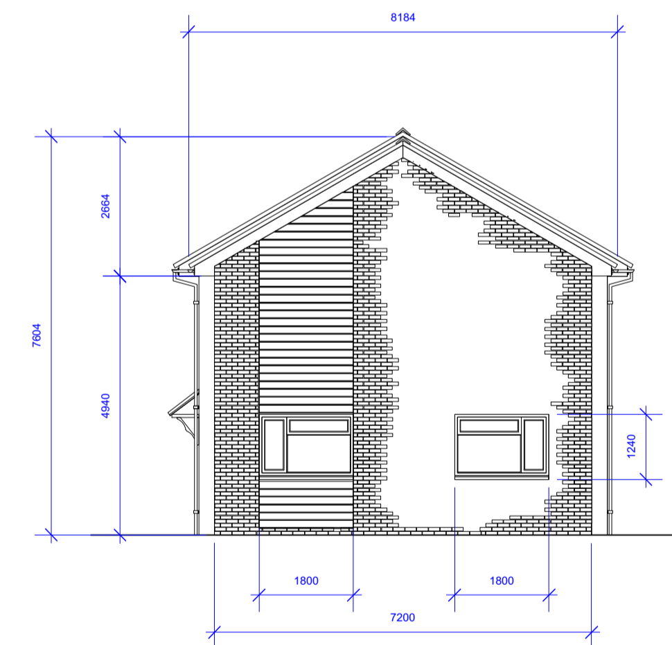
Proposed right hand side elevation Scale 1:100
