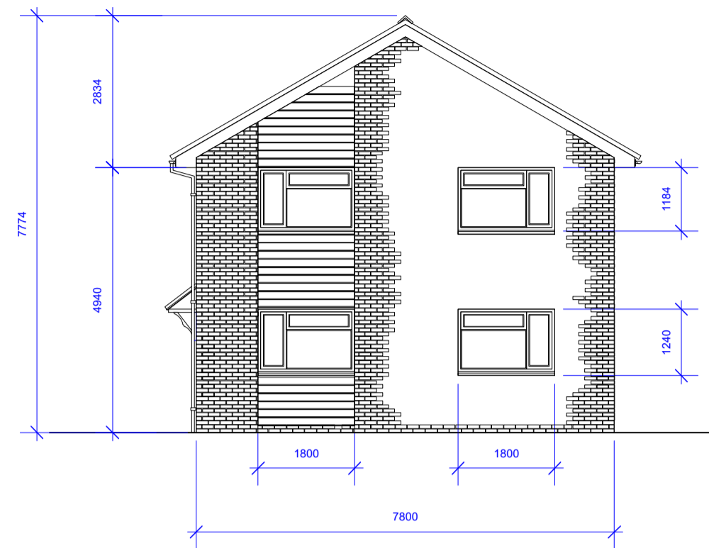
Existing right hand side elevation Scale 1:100
