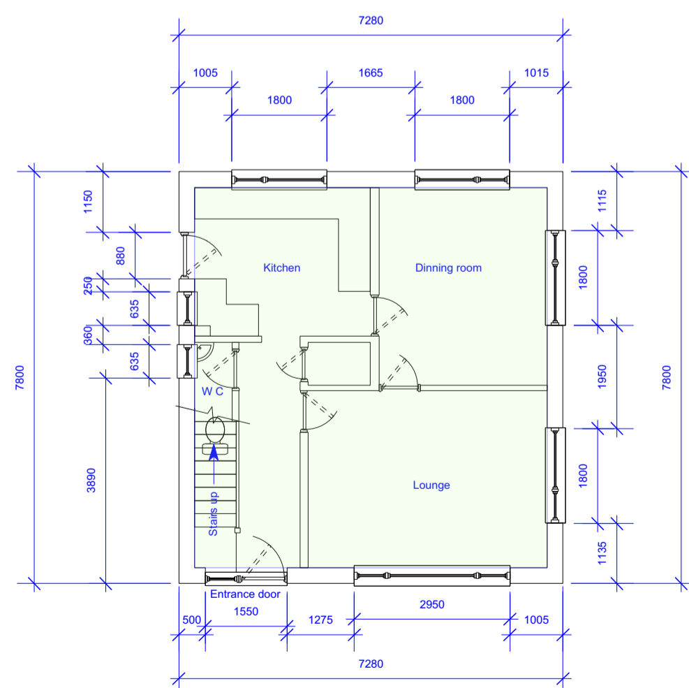
Existing ground floor Scale 1:100
