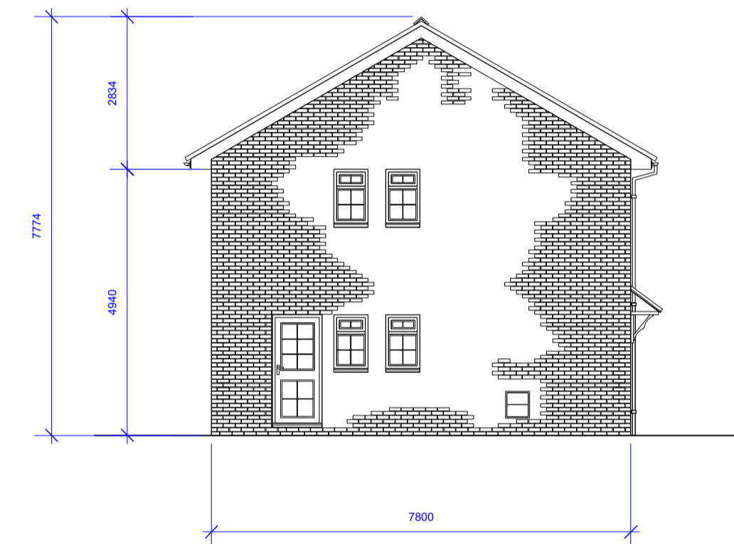
Existing left hand side elevation remains unchanged Scale 1:100
