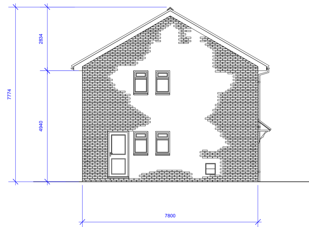
Existing left hand side elevation Scale 1:100
