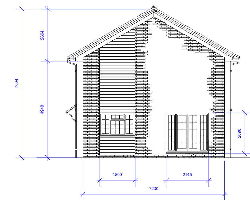
Proposed right hand side elevation Scale 1:100
