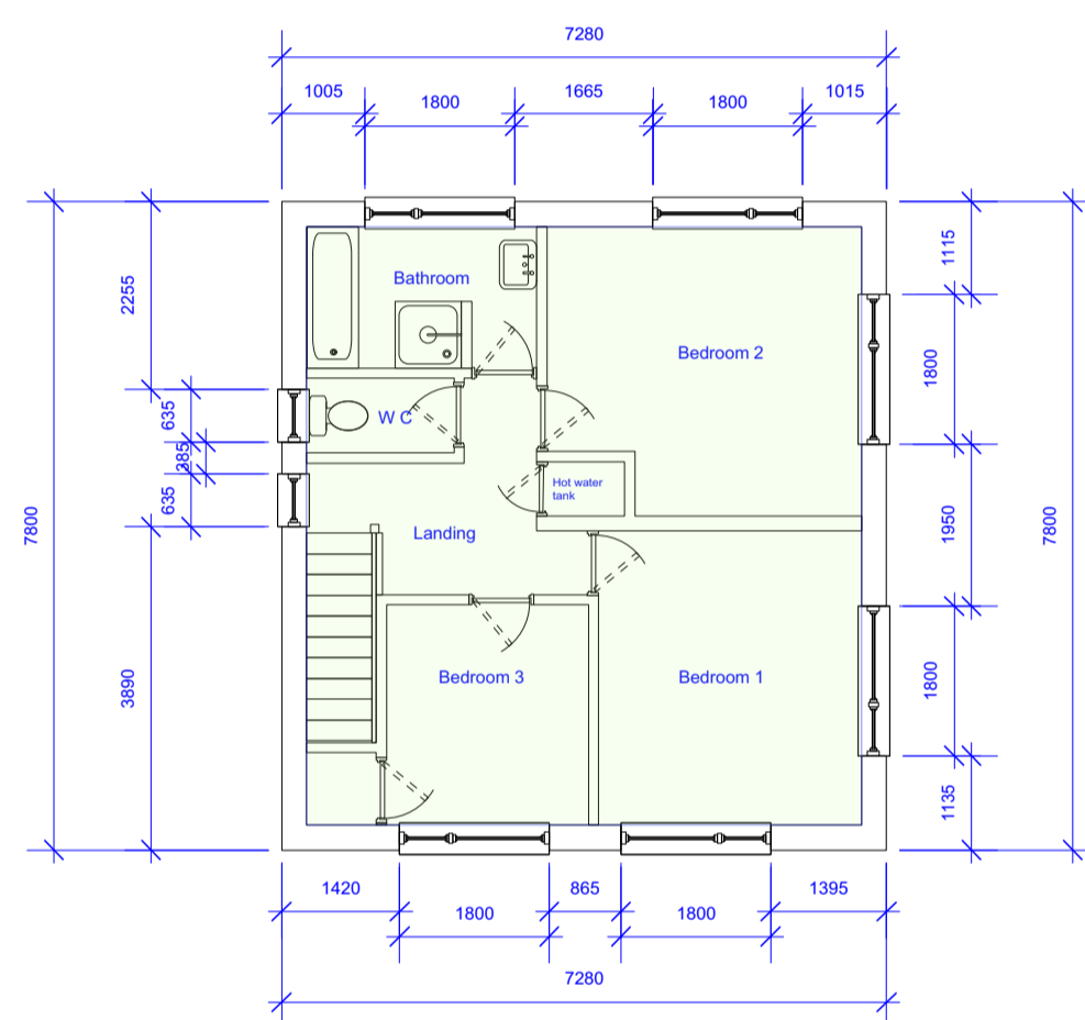
Existing first floor Scale 1:100
