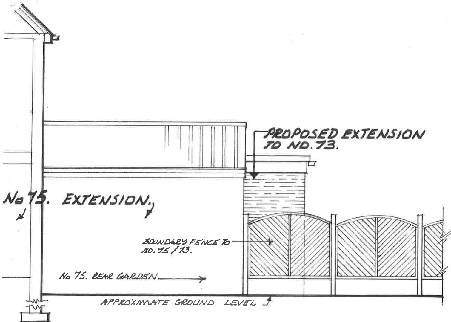
SIDE ELEVATION TO No. 75. WEST. PROPOSAL: SCHEME 'B' 04: EL: SCALE: - 1:50
