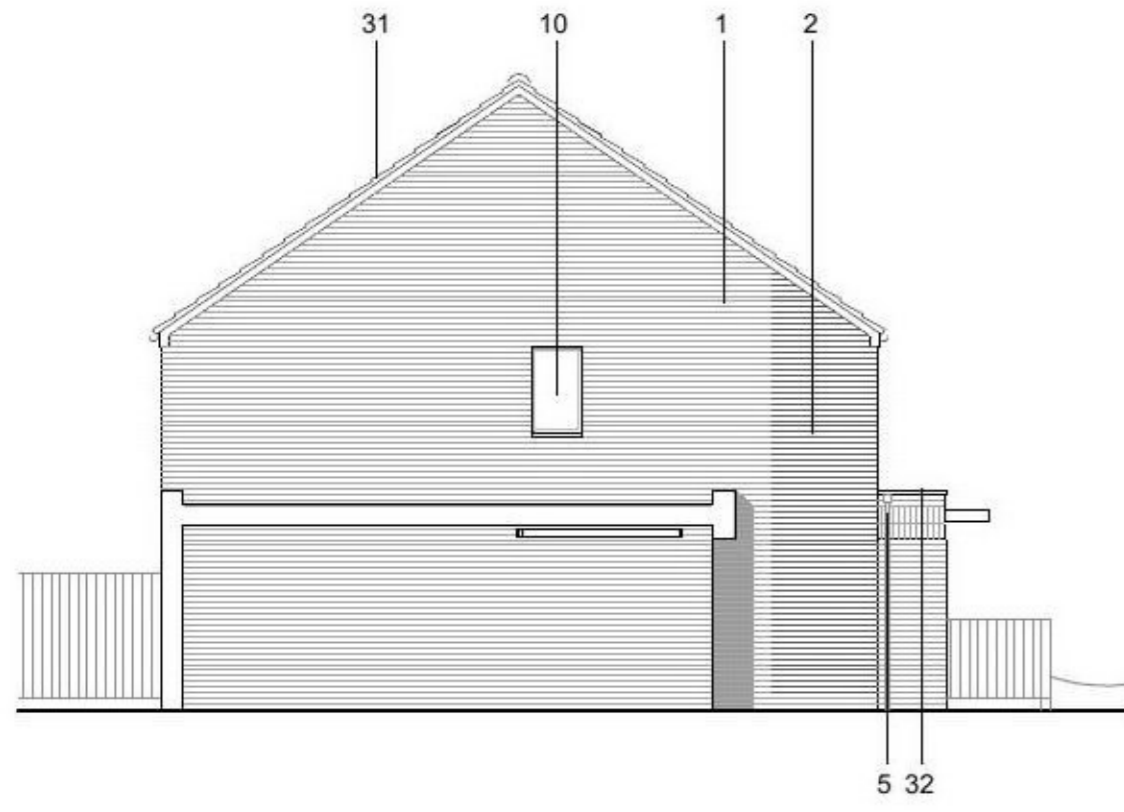
SIDE ELEVATION
