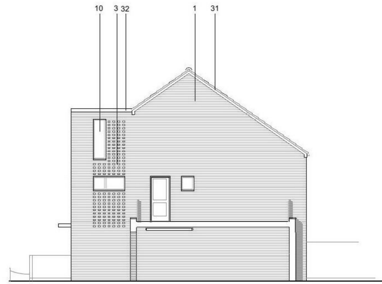
SIDE ELEVATION
