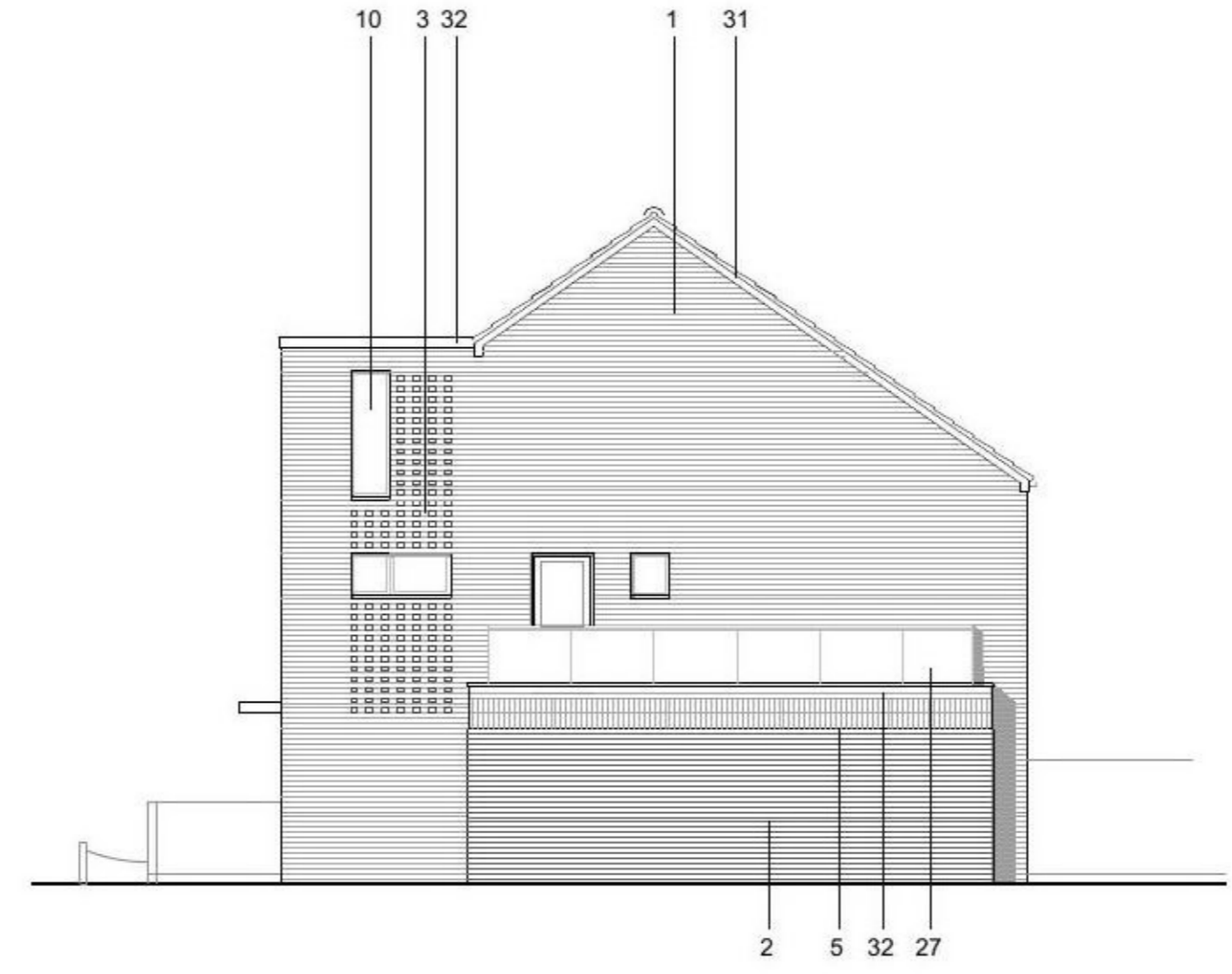
SIDE ELEVATION
