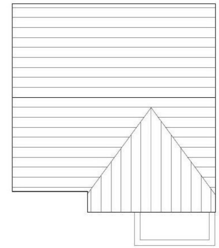
ROOF PLAN
