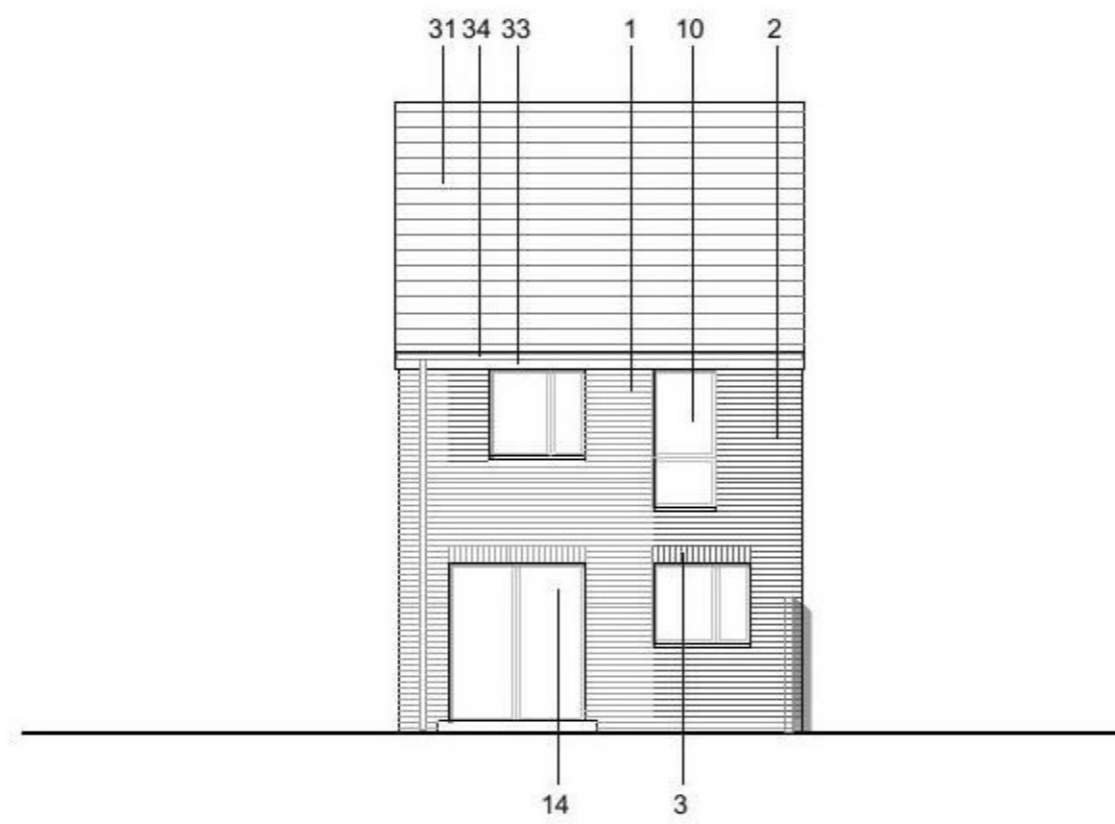
REAR ELEVATION
