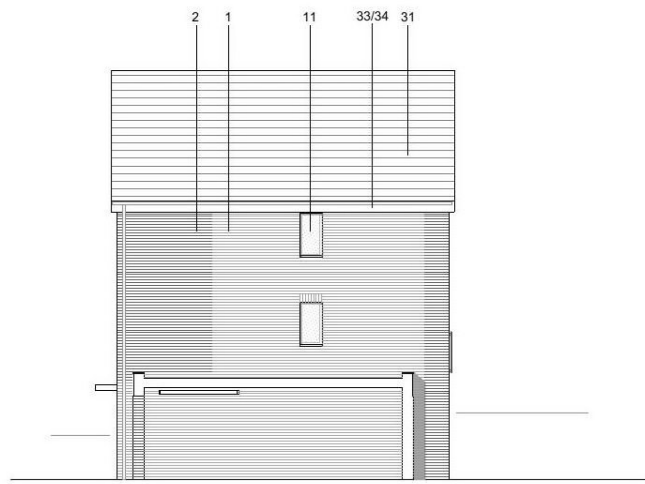
SIDE ELEVATION
