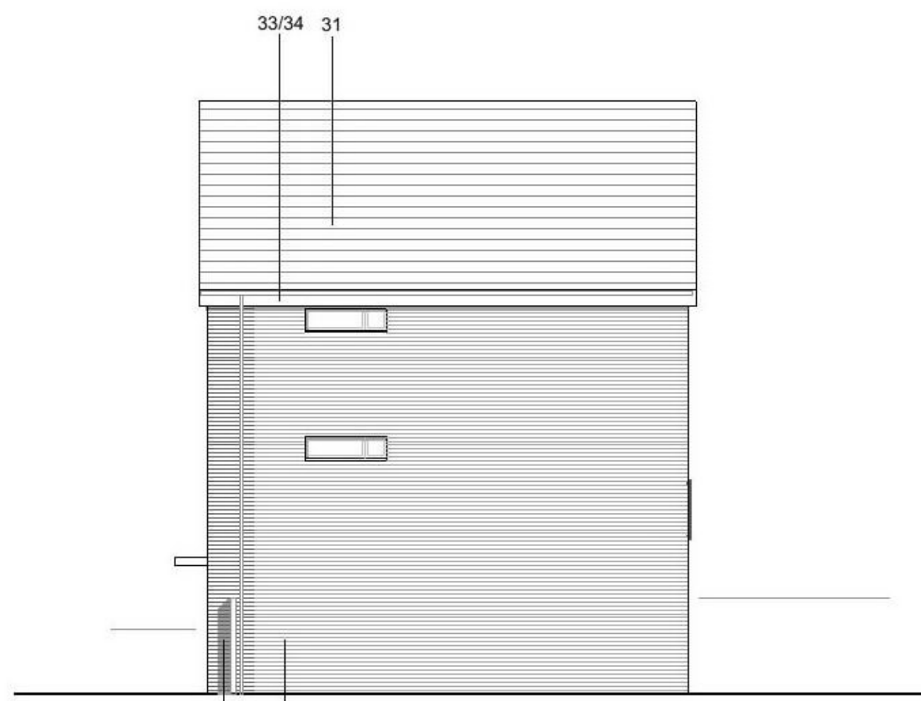
SIDE ELEVATION
