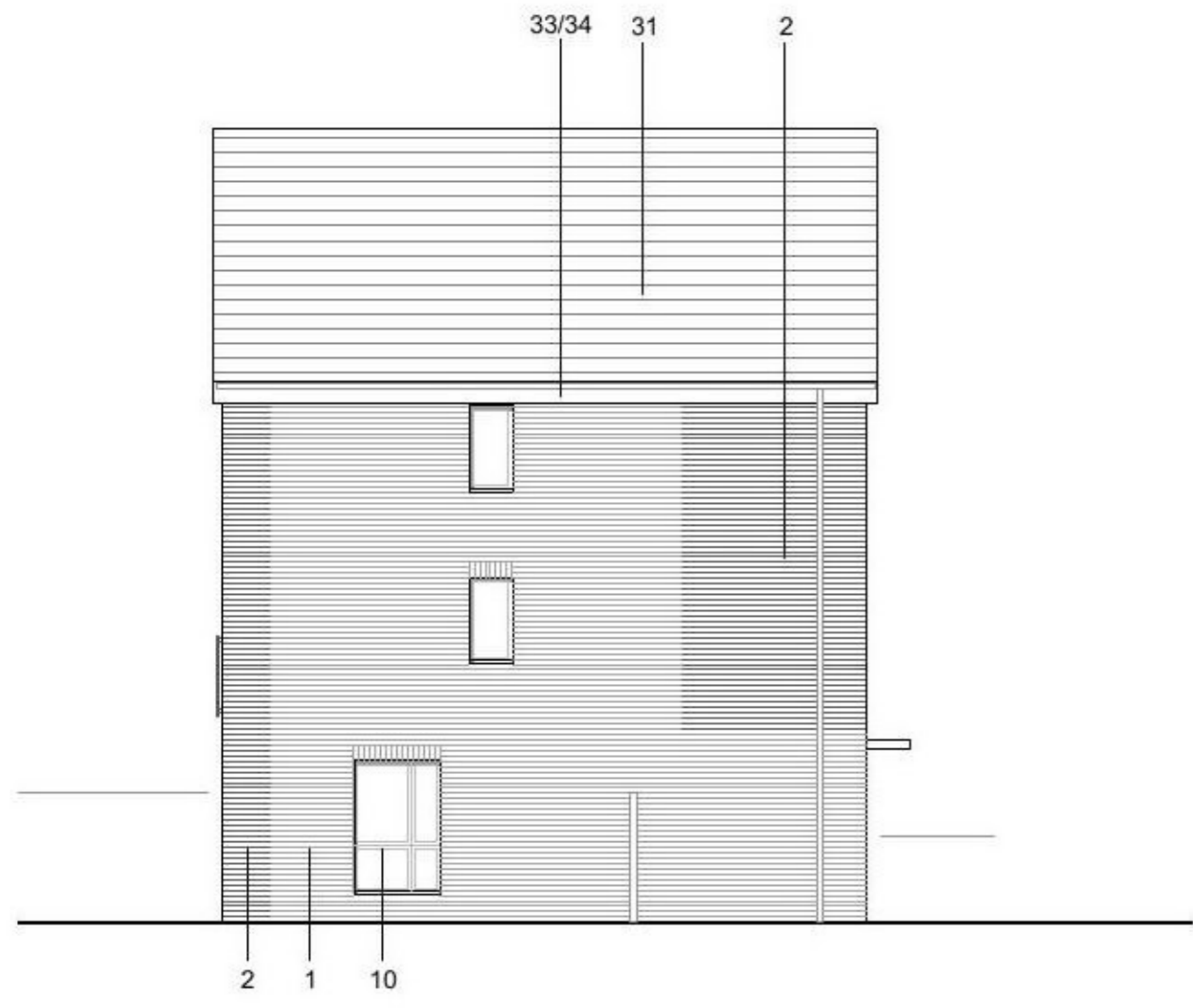
SIDE ELEVATION
