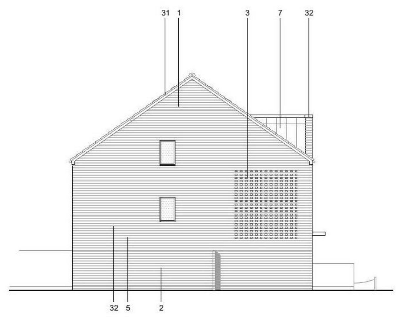
SIDE ELEVATION
