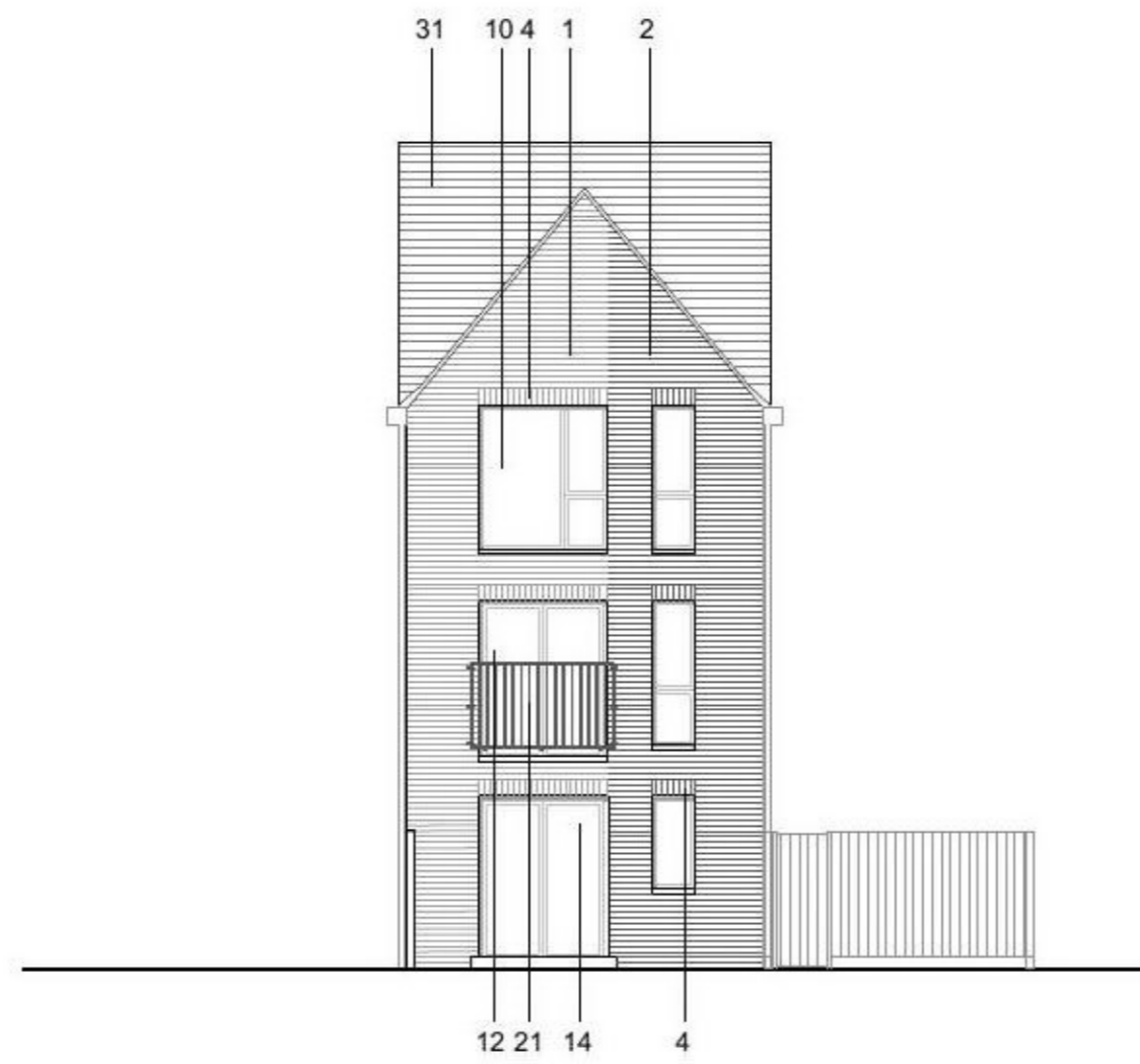
REAR ELEVATION
