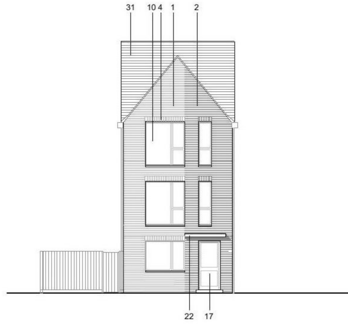
FRONT ELEVATION
