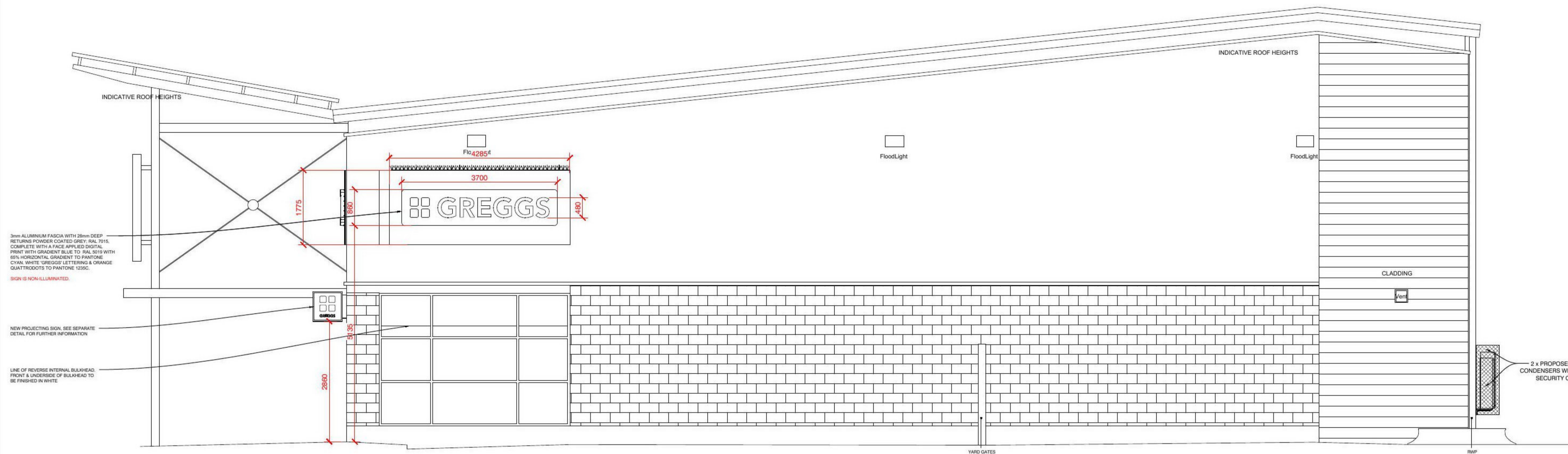
PROPOSED ELEVATION B-B
