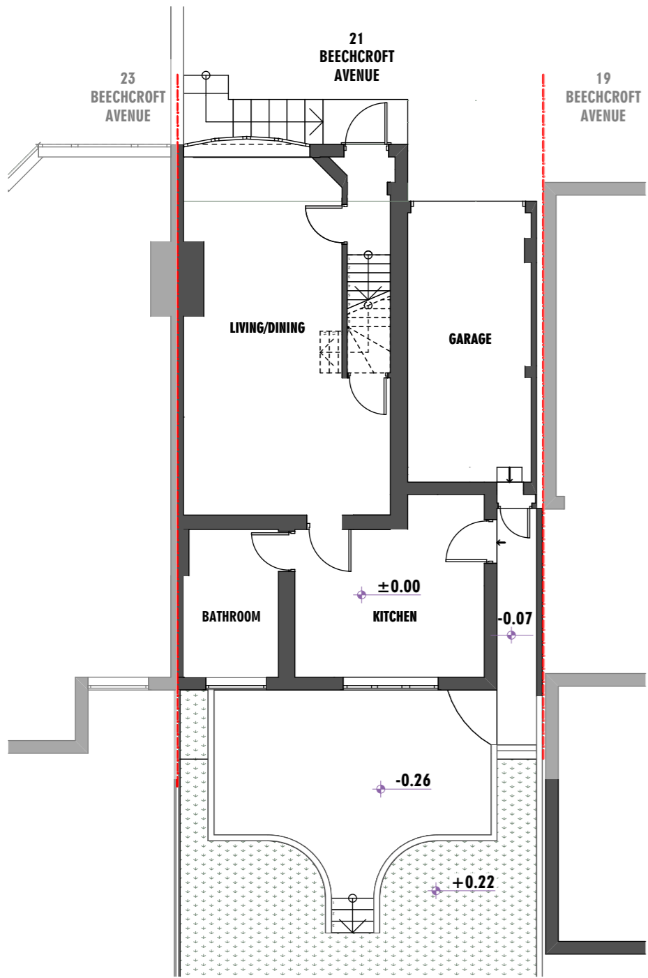
Ground Floor - Existing 1:100
