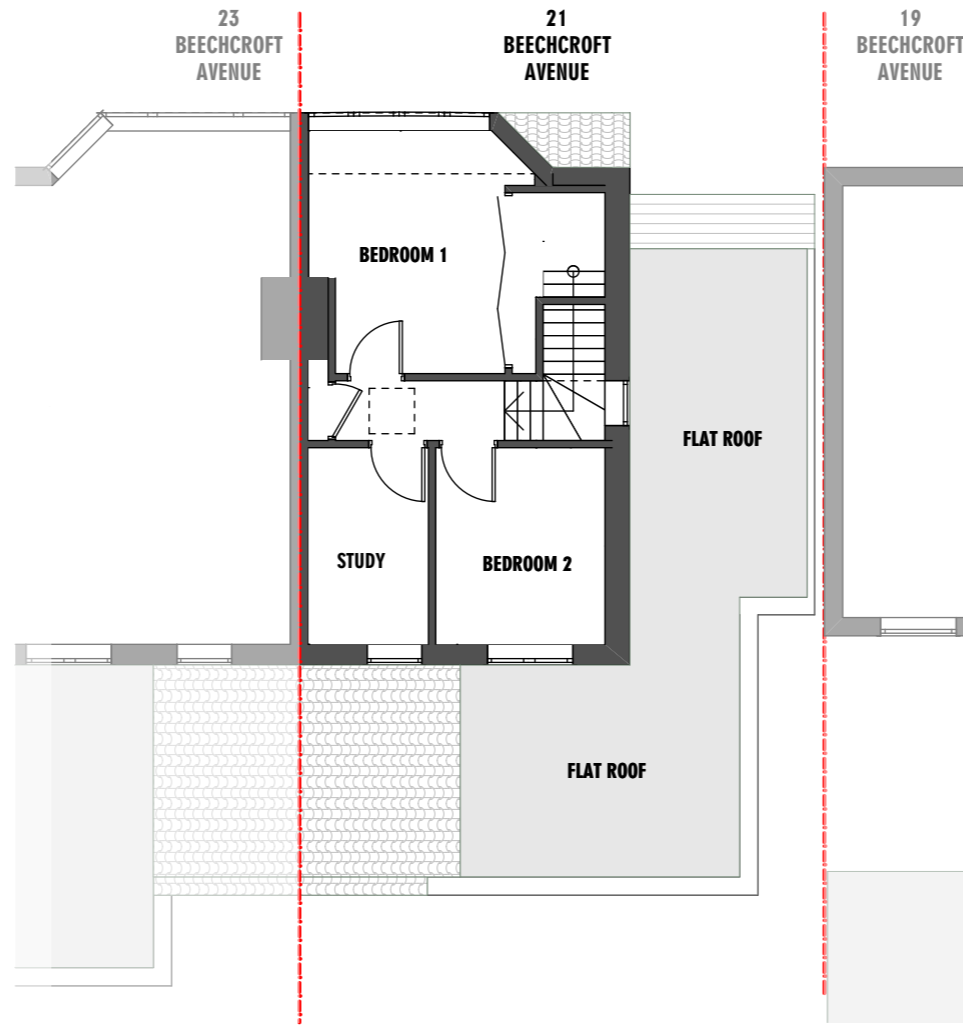
First Floor - Existing 1:100
