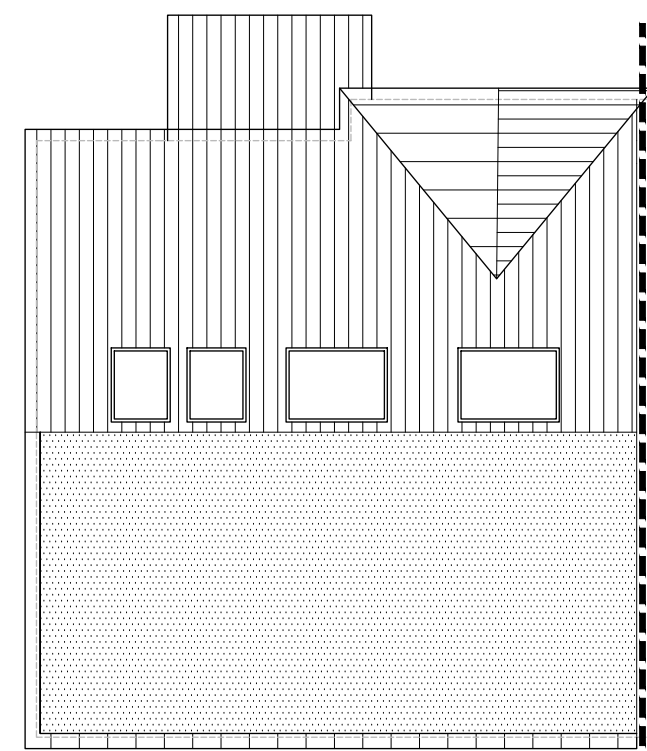
ROOF PLAN
