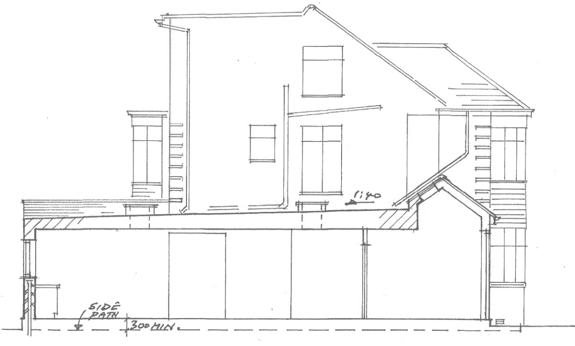
SECTION D-D PROPOSED
