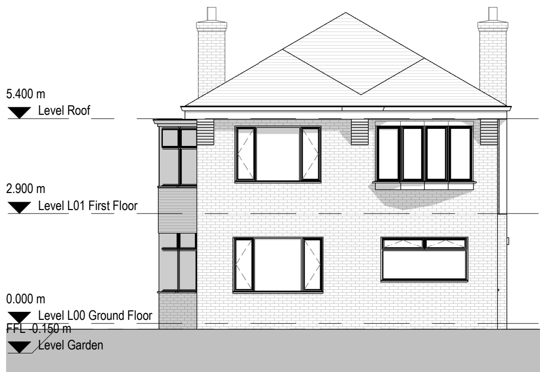
3 Existing South Elevation 1 : 100
