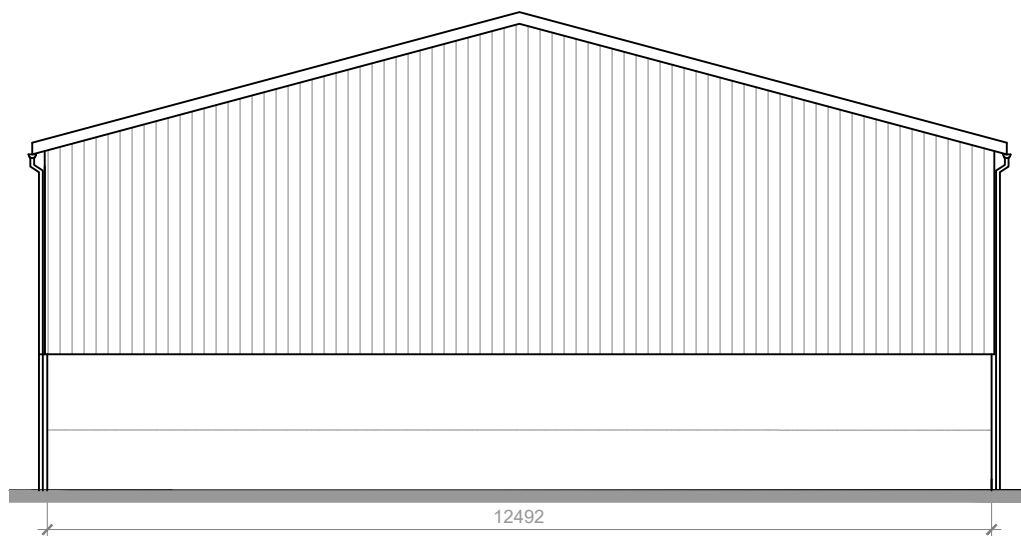
South Elevation
