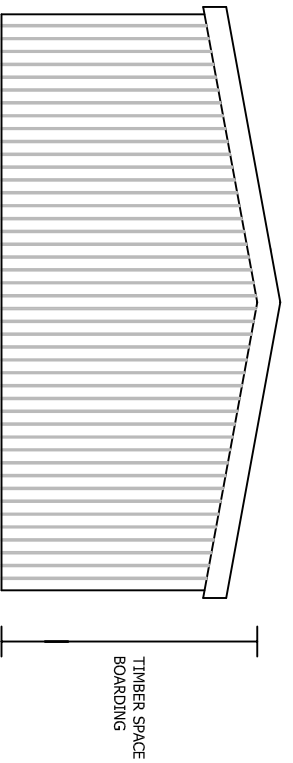
EAST ELEVATION
