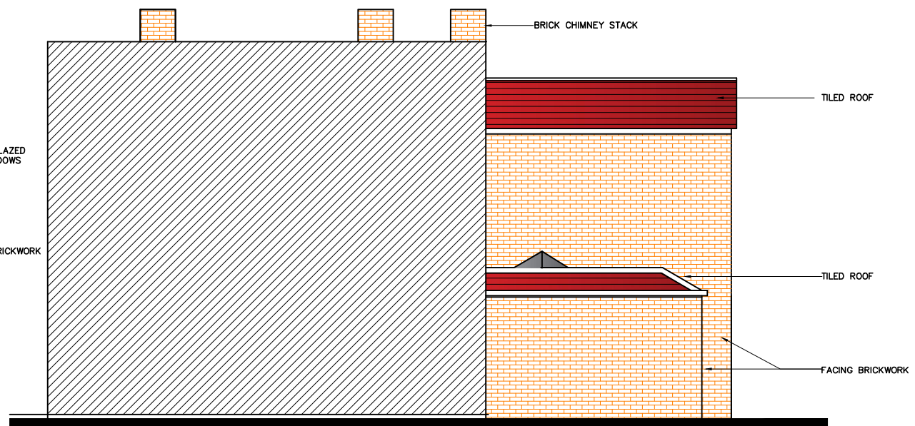
APPROVED WEST ELEVATION
