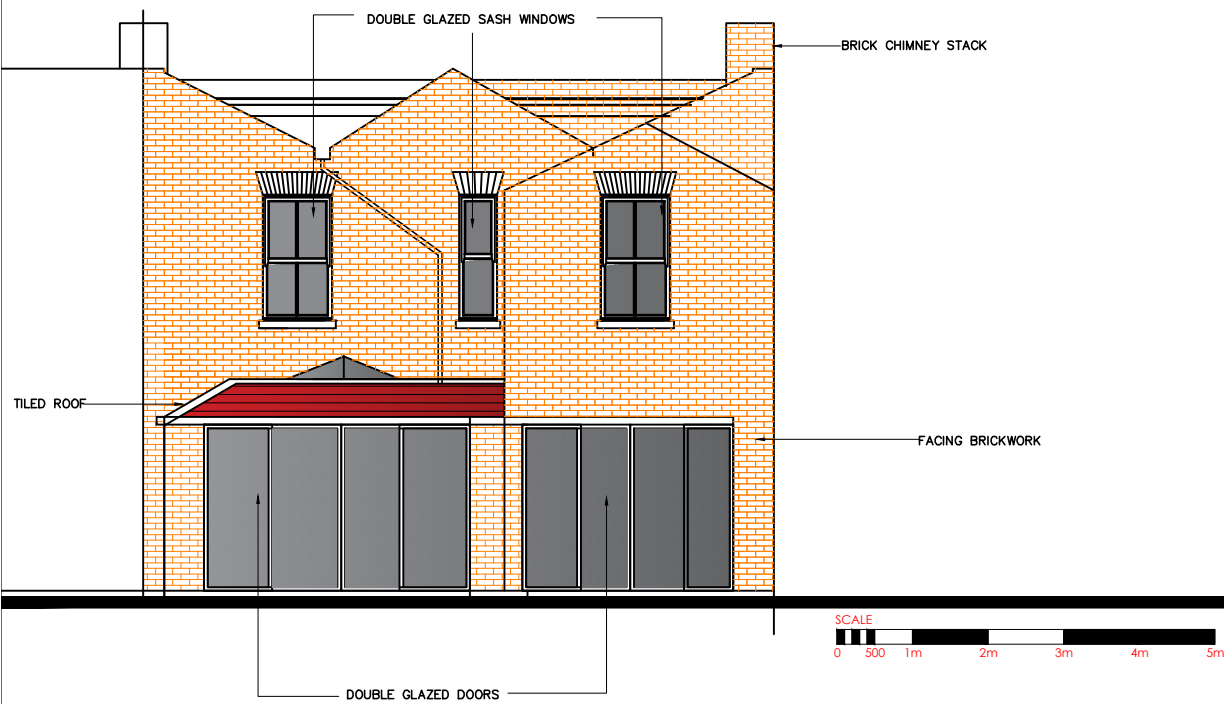
APPROVED REAR ELEVATION
