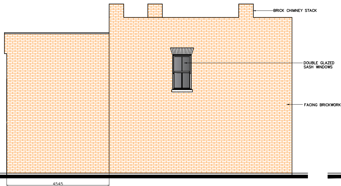
APPROVED EAST ELEVATION
