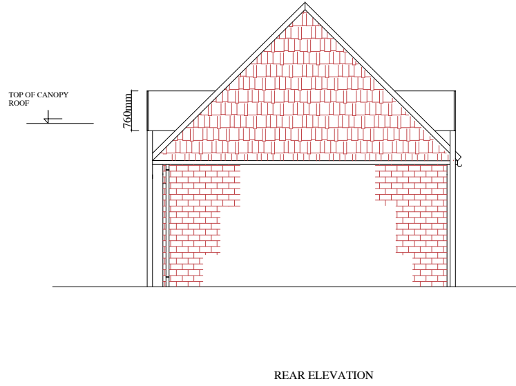
REAR ELEVATION
