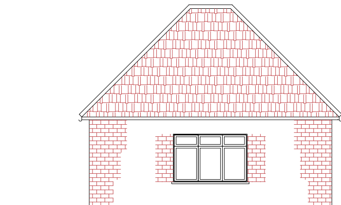
PRE EXISTING LEFT SIDE ELEVATION
