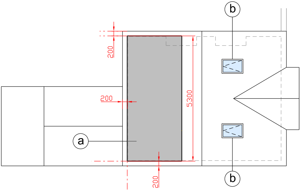
Roof Plan
