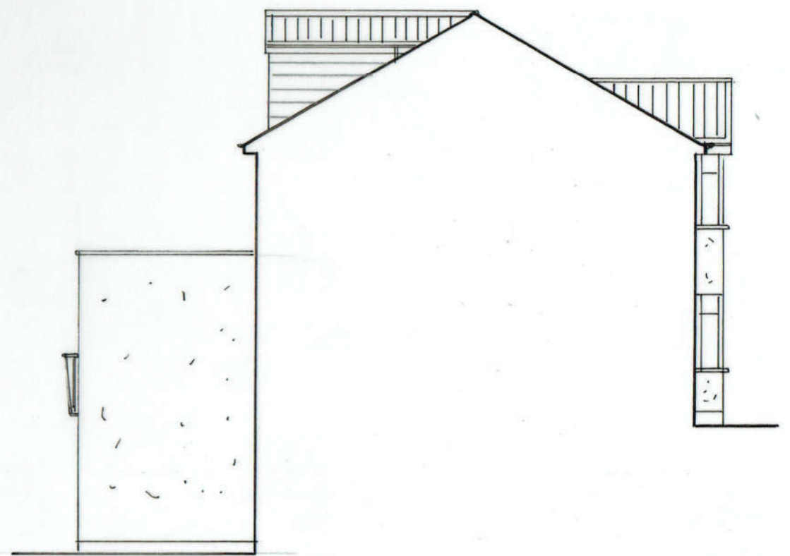
Proposed Side 'B' Elevation.
