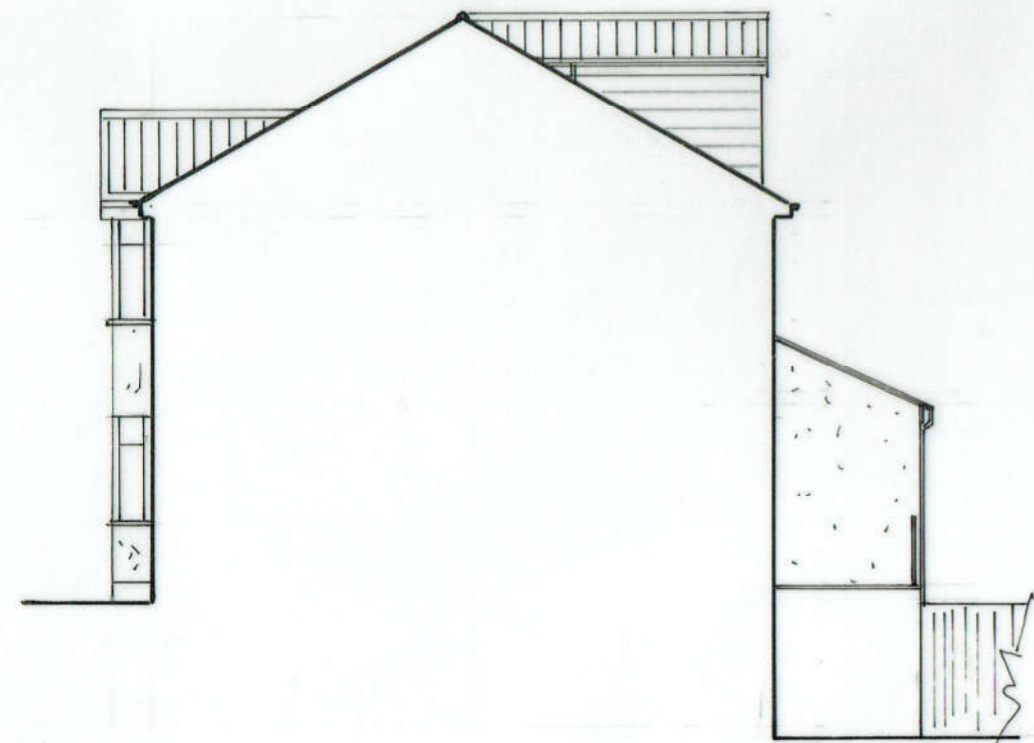
Existing Side 'A' Elevation.
