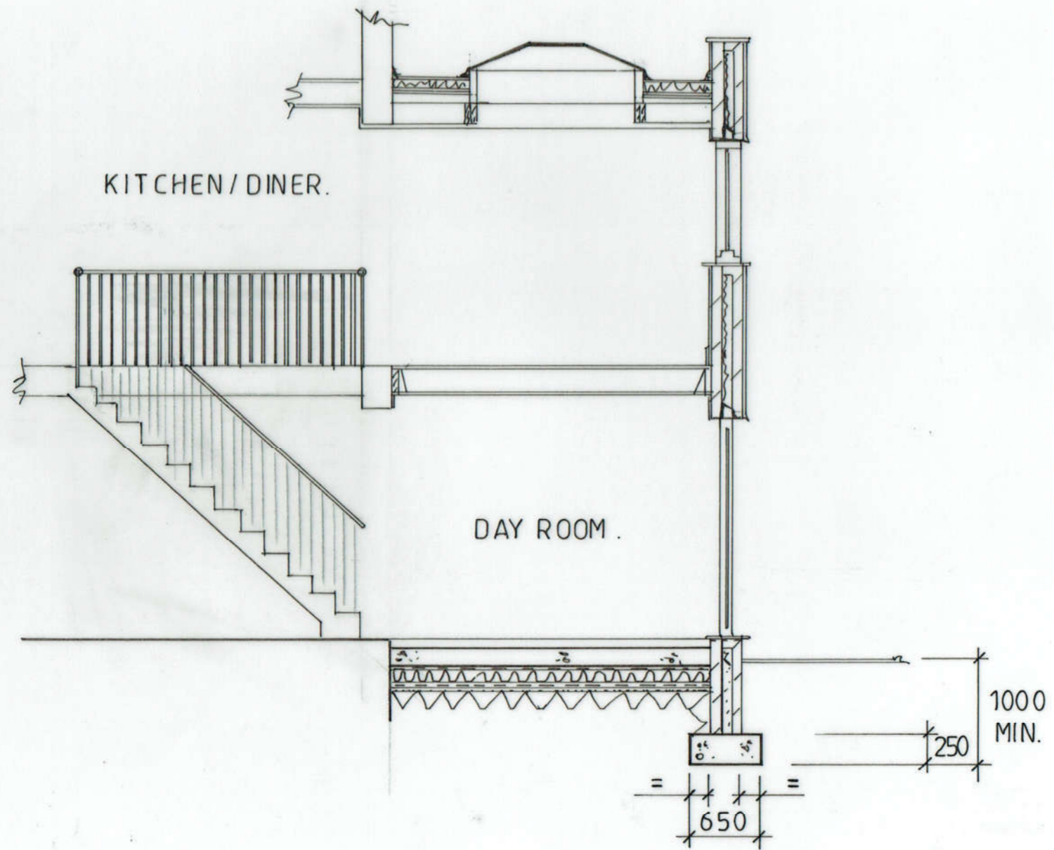
TYPICAL SECTION.
