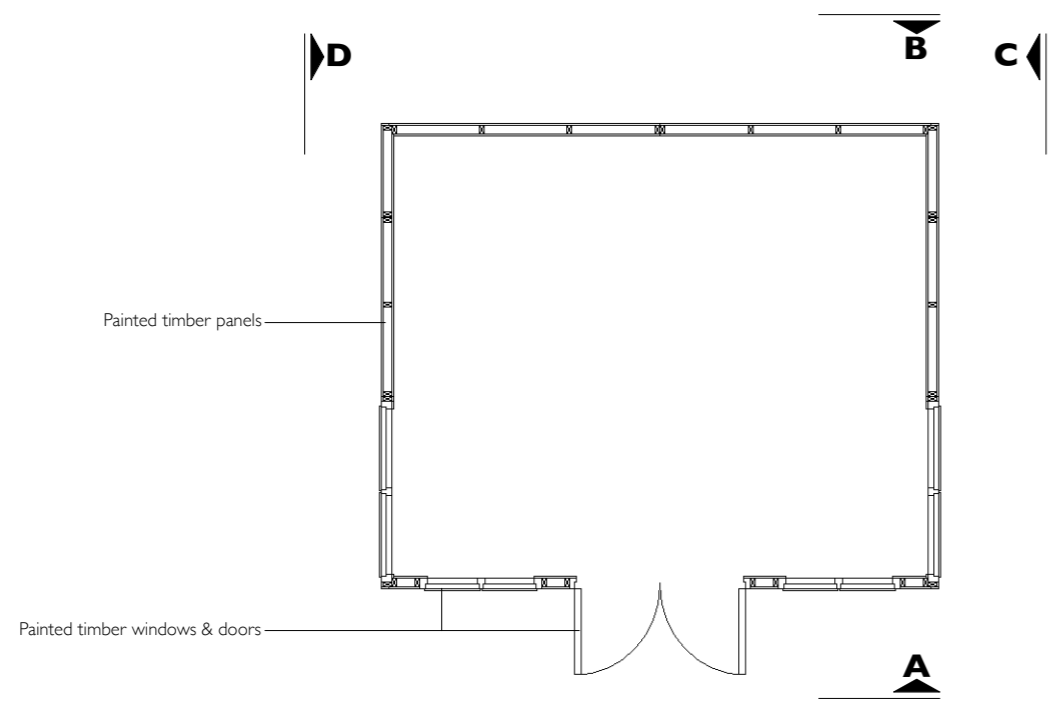
1 GARDEN ROOM PLAN 1:50 @ A3
