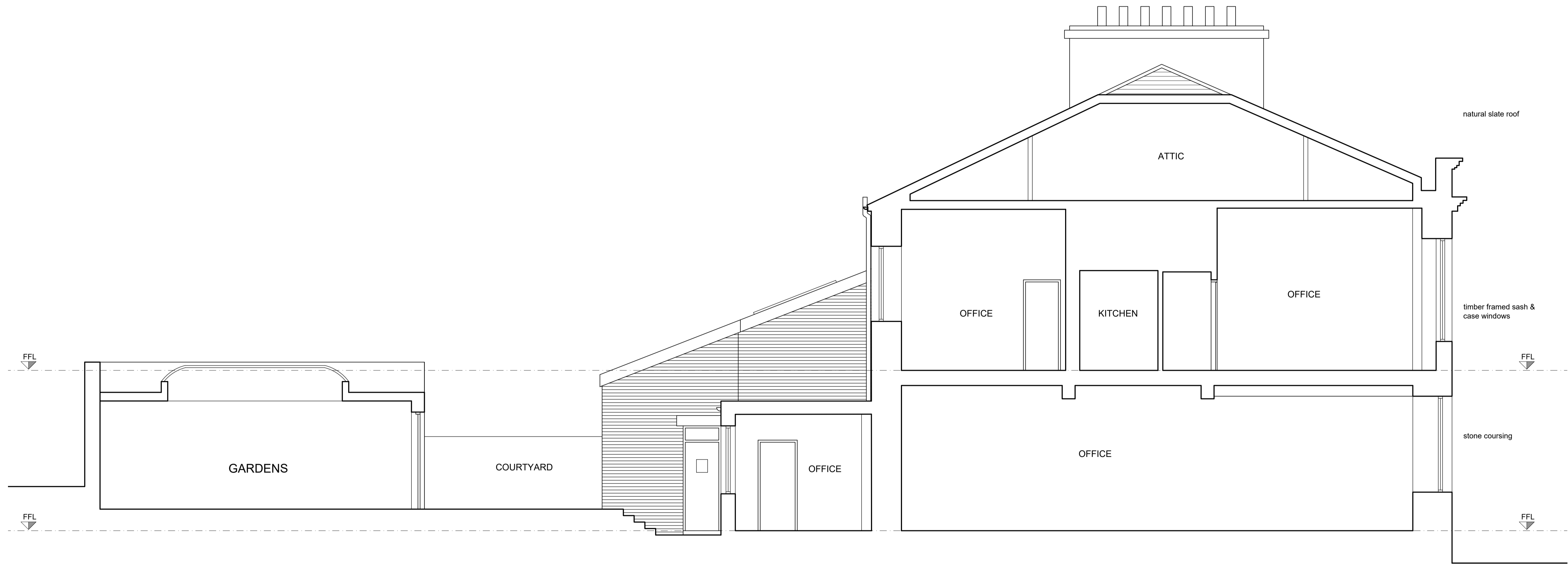
SECTION A-A AS EXISTING
